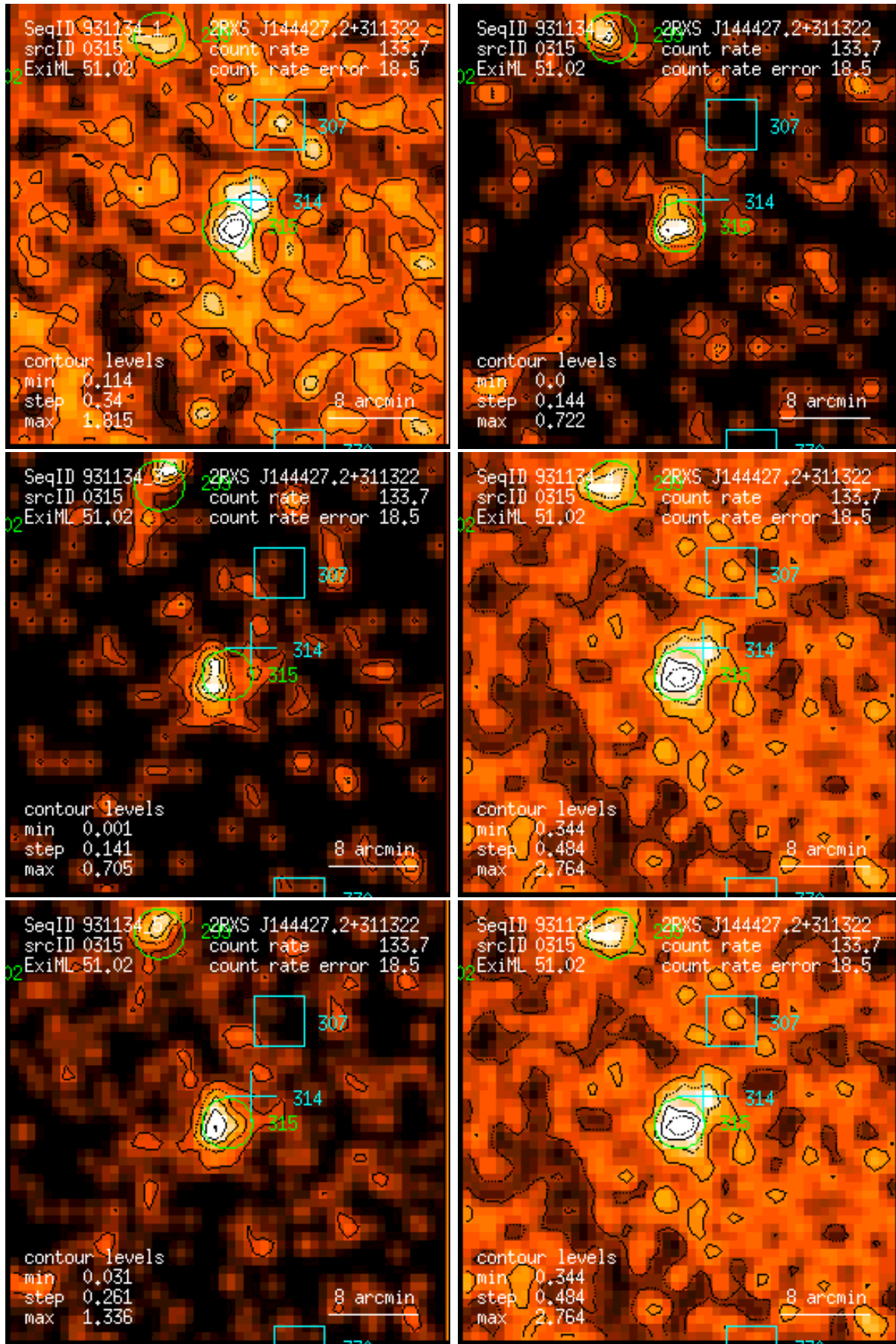
Figure 315: RASS 931134: detection 0315: band rate images, Gaussian filter: (1) PSPC channels 11 – 41, (2) 52 – 90, (3) 91 – 201, (4) 11 – 235, (5) 52 – 201, (6) 11 – 201. Broad band rates in counts/ks. Band rate contour levels in counts/ks/arcmin 2 .
