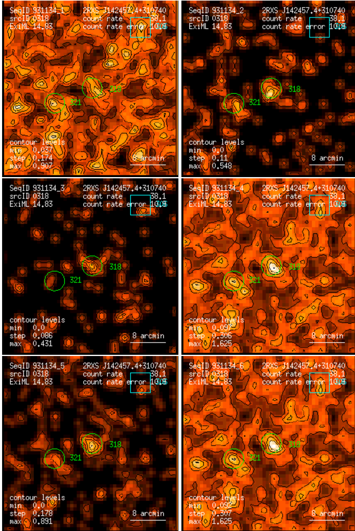
Figure 318: RASS 931134: detection 0318: band rate images, Gaussian filter: (1) PSPC channels 11 – 41, (2) 52 – 90, (3) 91 – 201, (4) 11 – 235, (5) 52 – 201, (6) 11 – 201. Broad band rates in counts/ks. Band rate contour levels in counts/ks/arcmin 2 .
