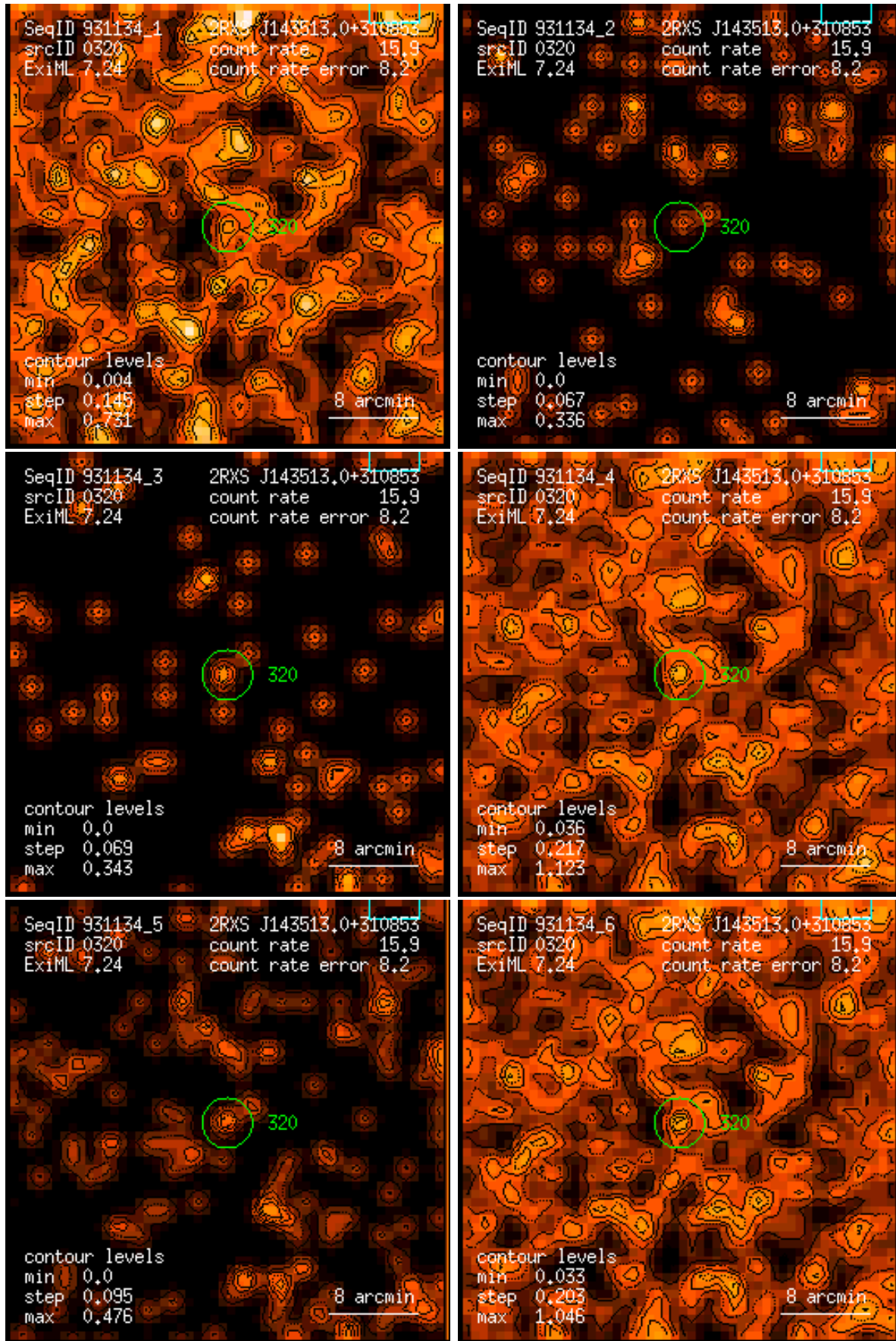
Figure 320: RASS 931134: detection 0320: band rate images, Gaussian filter: (1) PSPC channels 11 – 41, (2) 52 – 90, (3) 91 – 201, (4) 11 – 235, (5) 52 – 201, (6) 11 – 201. Broad band rates in counts/ks. Band rate contour levels in counts/ks/arcmin 2 .
