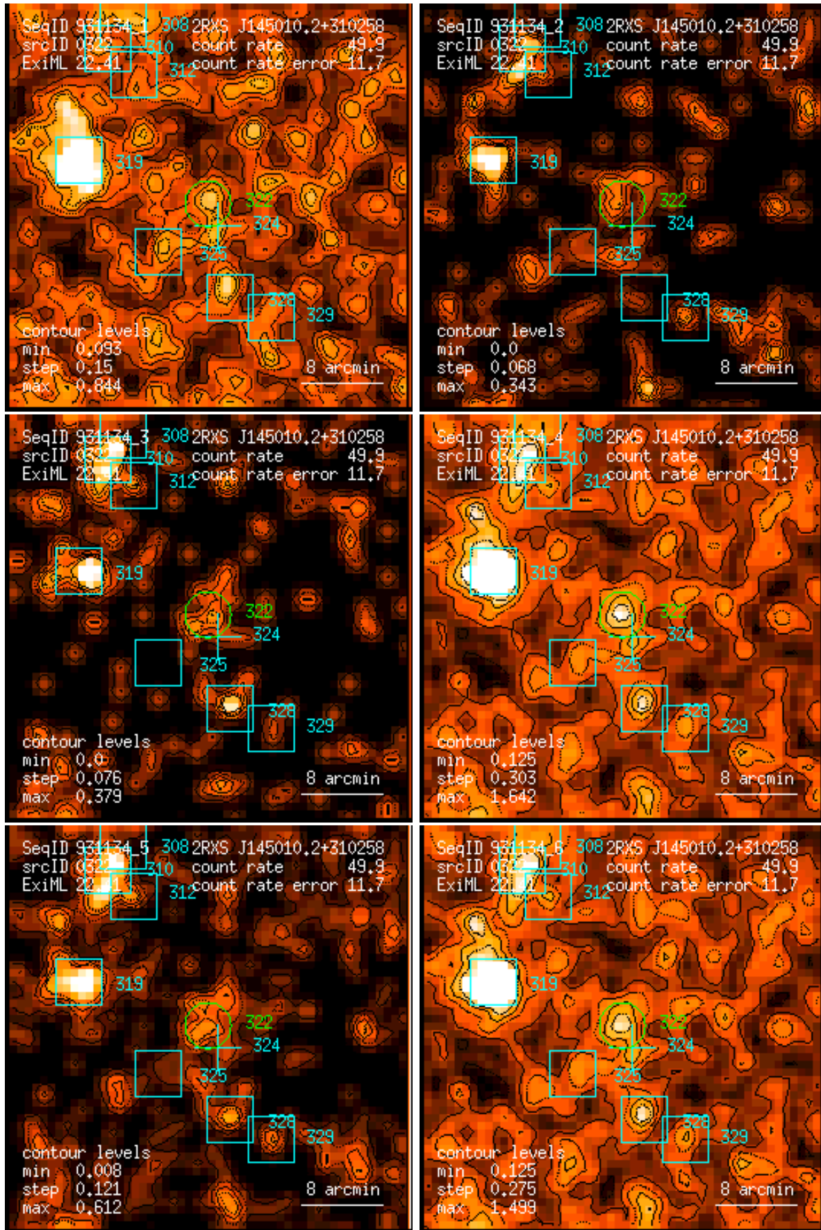
Figure 322: RASS 931134: detection 0322: band rate images, Gaussian filter: (1) PSPC channels 11 – 41, (2) 52 – 90, (3) 91 – 201, (4) 11 – 235, (5) 52 – 201, (6) 11 – 201. Broad band rates in counts/ks. Band rate contour levels in counts/ks/arcmin 2 .
