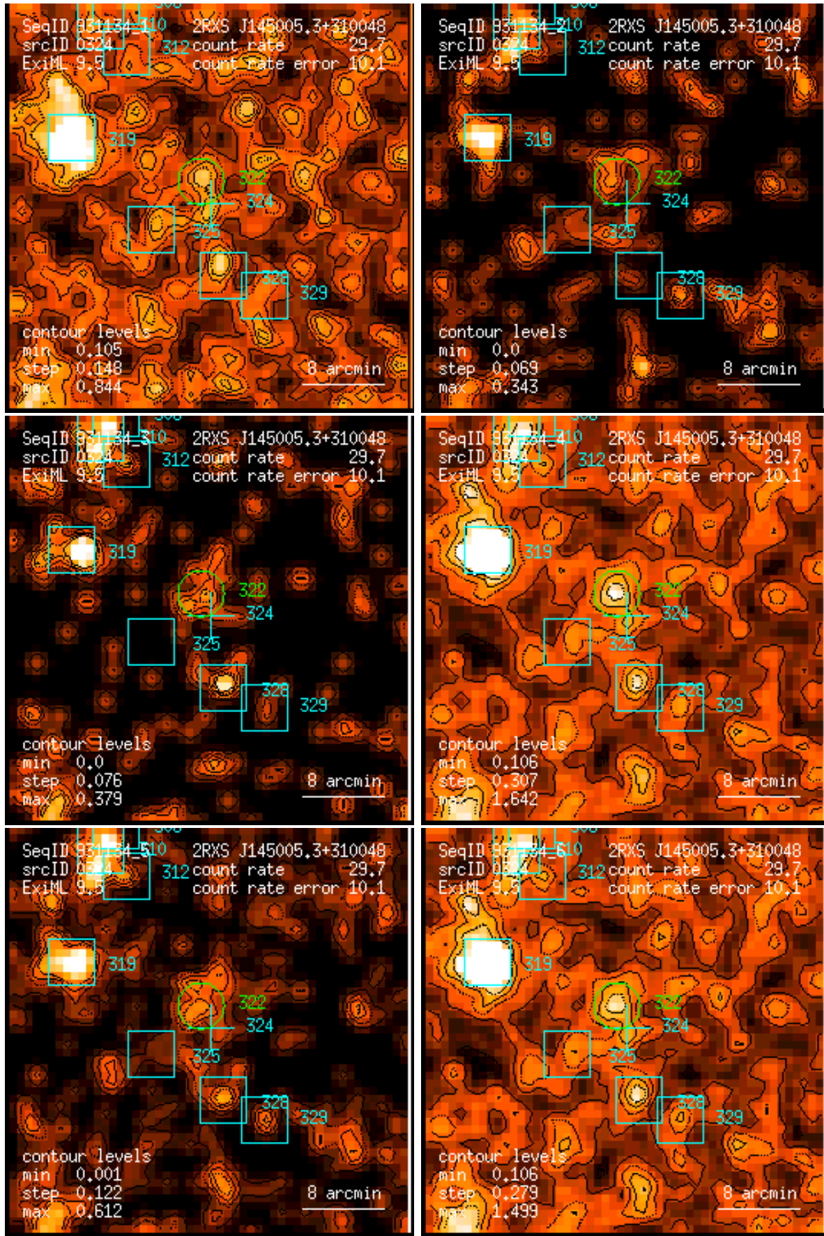
Figure 324: RASS 931134: detection 0324: band rate images, Gaussian filter: (1) PSPC channels 11 – 41, (2) 52 – 90, (3) 91 – 201, (4) 11 – 235, (5) 52 – 201, (6) 11 – 201. Broad band rates in counts/ks. Band rate contour levels in counts/ks/arcmin 2 .
