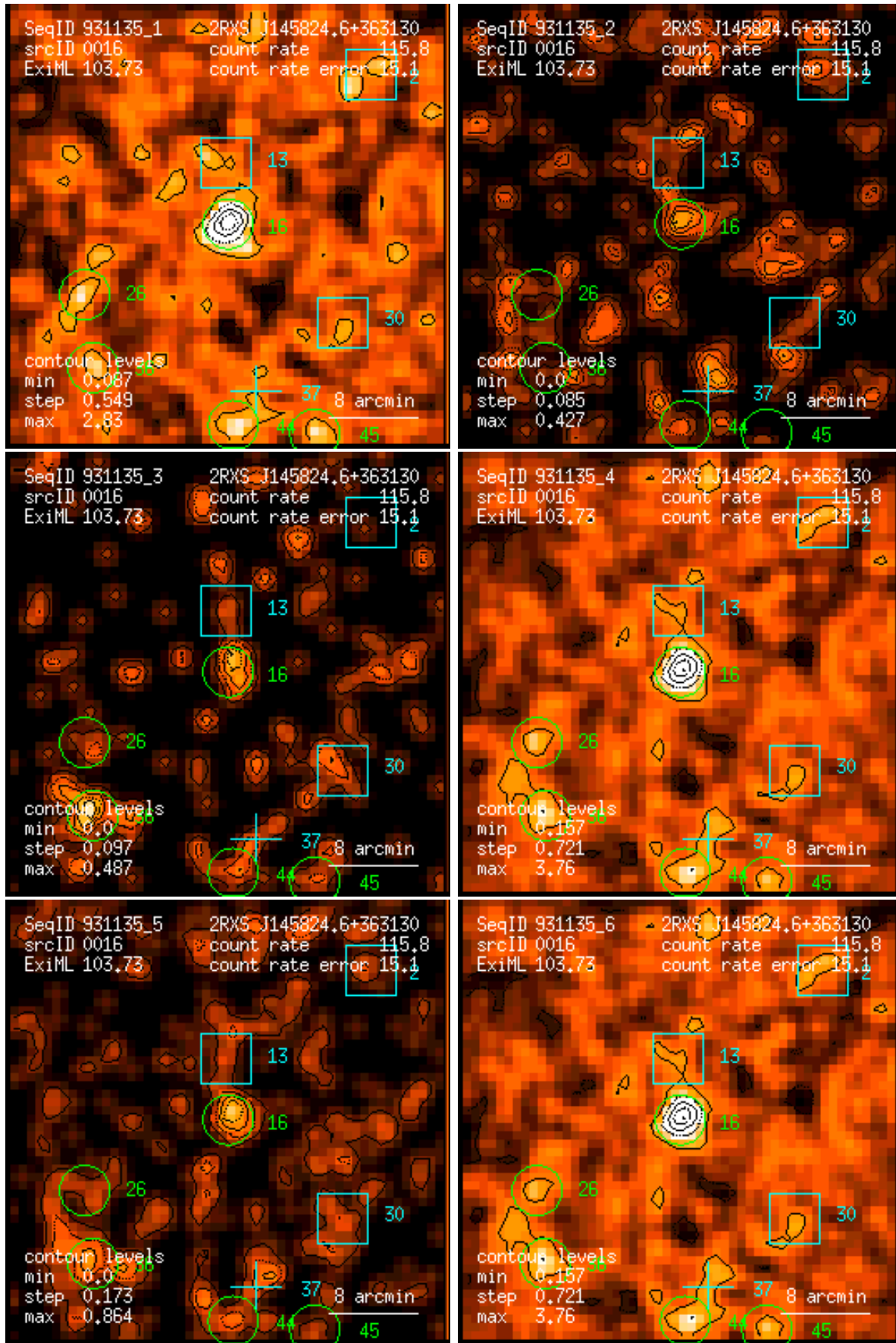
Figure 16: RASS 931135: detection 0016: band rate images, Gaussian filter: (1) PSPC channels 11 – 41, (2) 52 – 90, (3) 91 – 201, (4) 11 – 235, (5) 52 – 201, (6) 11 – 201. Broad band rates in counts/ks. Band rate contour levels in counts/ks/arcmin 2 .
