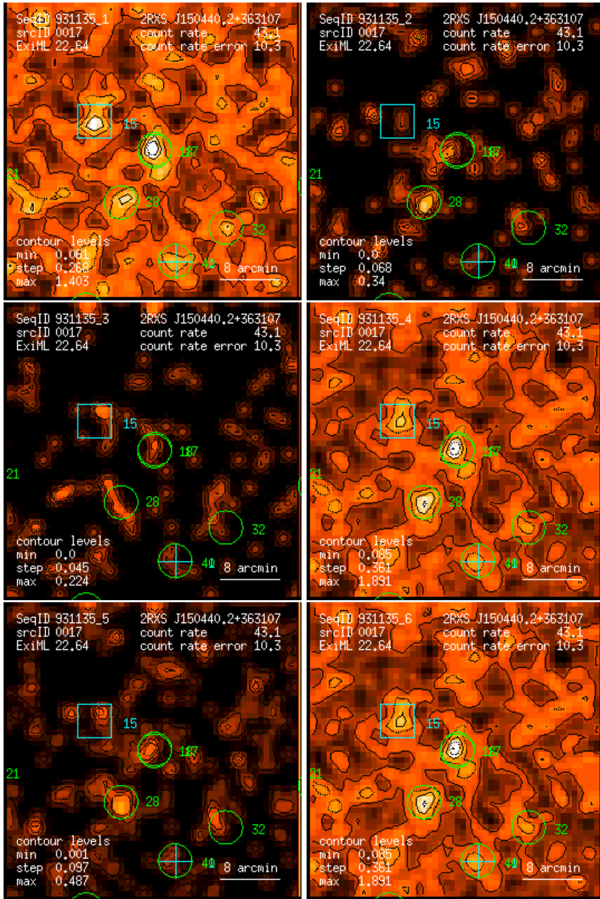
Figure 17: RASS 931135: detection 0017: band rate images, Gaussian filter: (1) PSPC channels 11 – 41, (2) 52 – 90, (3) 91 – 201, (4) 11 – 235, (5) 52 – 201, (6) 11 – 201. Broad band rates in counts/ks. Band rate contour levels in counts/ks/arcmin 2 .
