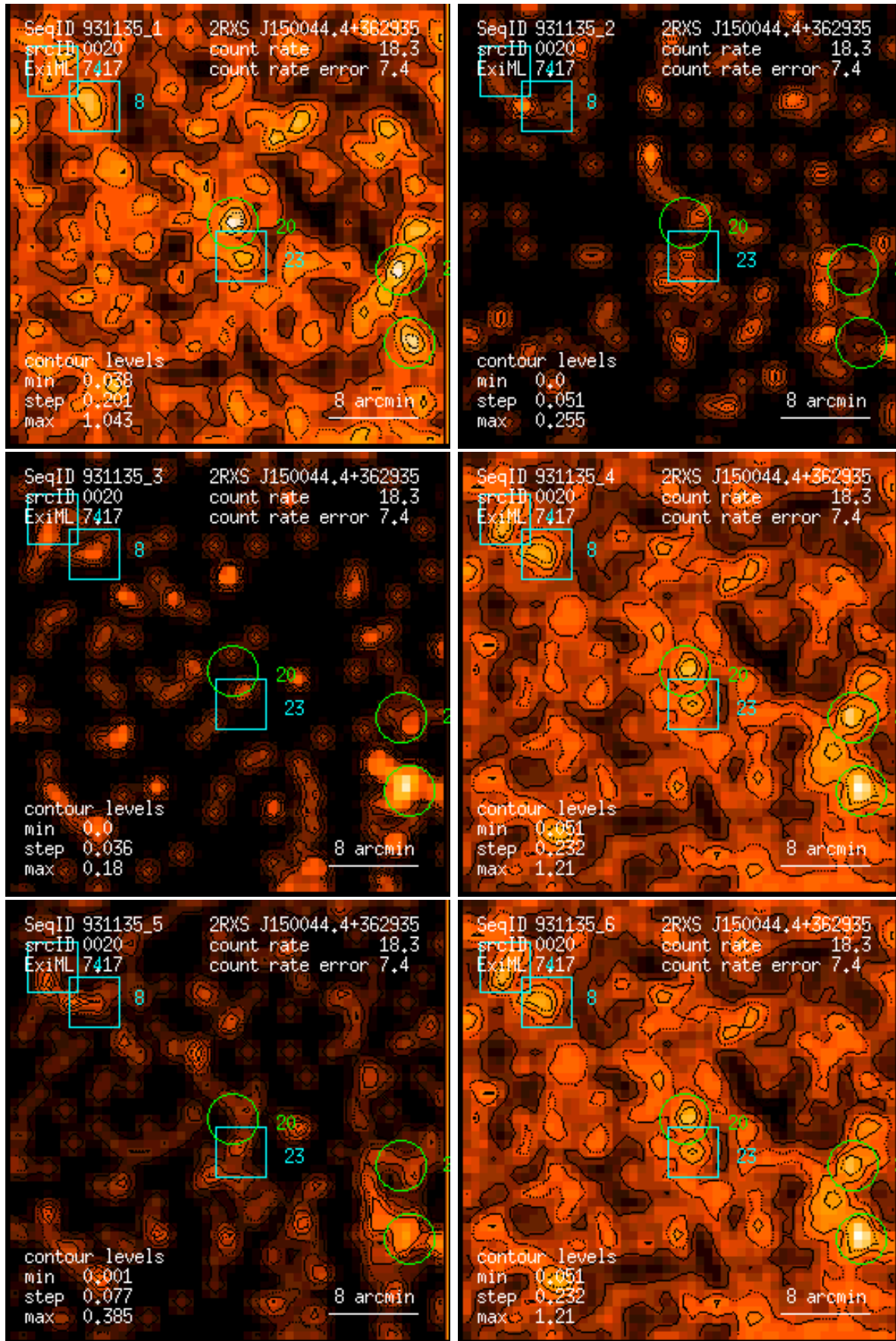
Figure 20: RASS 931135: detection 0020: band rate images, Gaussian filter: (1) PSPC channels 11 – 41, (2) 52 – 90, (3) 91 – 201, (4) 11 – 235, (5) 52 – 201, (6) 11 – 201. Broad band rates in counts/ks. Band rate contour levels in counts/ks/arcmin 2 .
