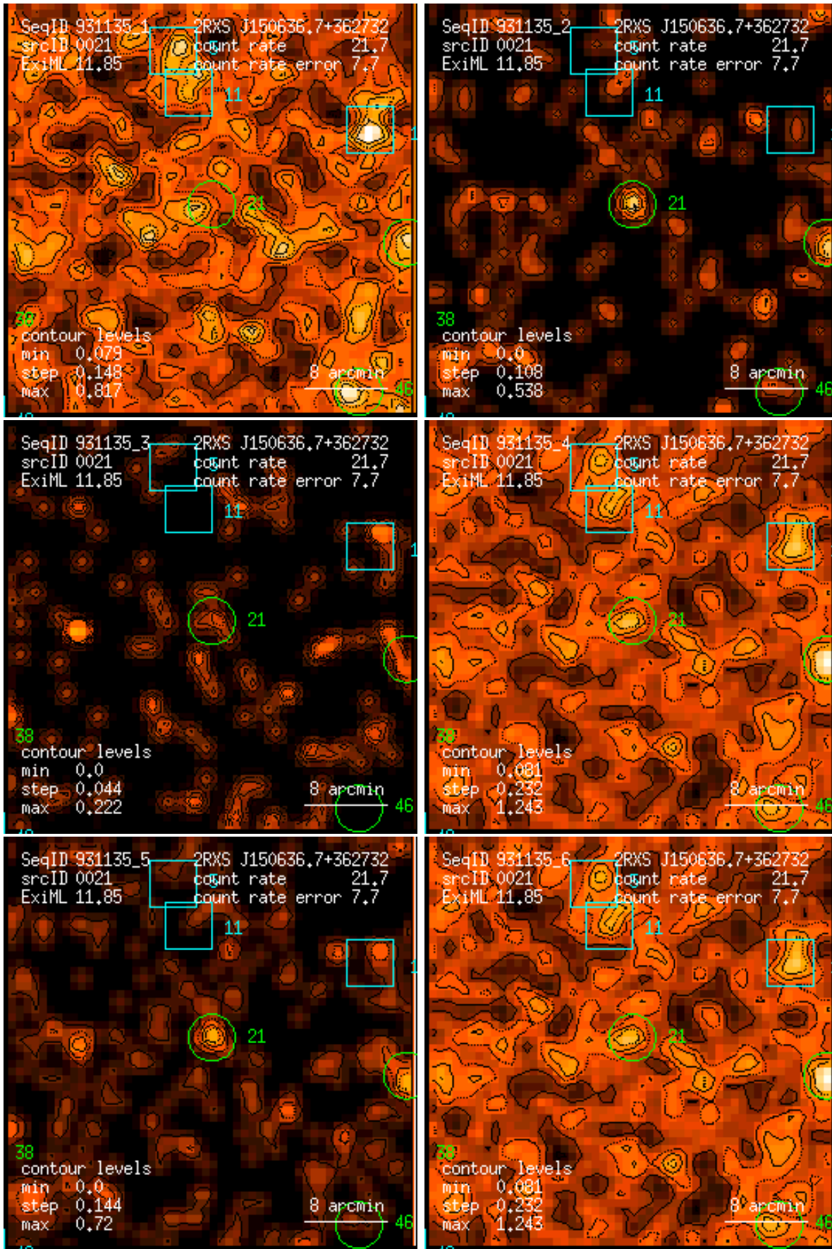
Figure 21: RASS 931135: detection 0021: band rate images, Gaussian filter: (1) PSPC channels 11 – 41, (2) 52 – 90, (3) 91 – 201, (4) 11 – 235, (5) 52 – 201, (6) 11 – 201. Broad band rates in counts/ks. Band rate contour levels in counts/ks/arcmin 2 .
