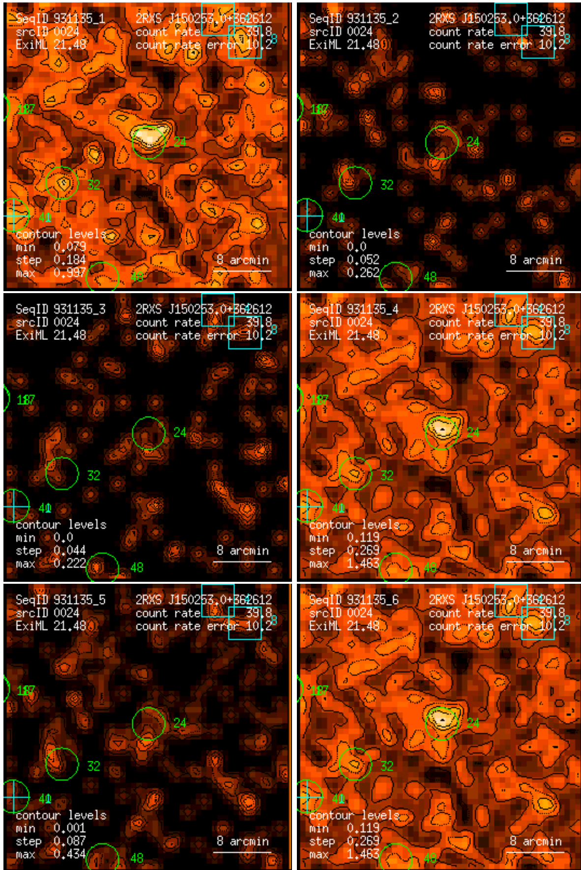
Figure 24: RASS 931135: detection 0024: band rate images, Gaussian filter: (1) PSPC channels 11 – 41, (2) 52 – 90, (3) 91 – 201, (4) 11 – 235, (5) 52 – 201, (6) 11 – 201. Broad band rates in counts/ks. Band rate contour levels in counts/ks/arcmin 2 .
