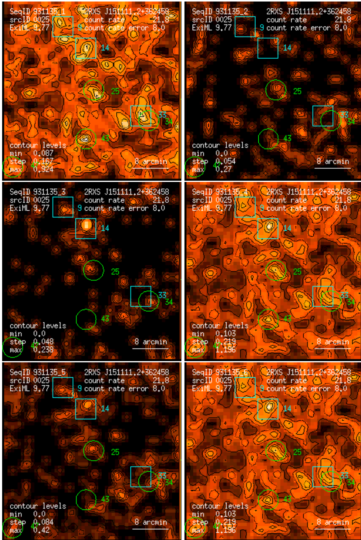
Figure 25: RASS 931135: detection 0025: band rate images, Gaussian filter: (1) PSPC channels 11 – 41, (2) 52 – 90, (3) 91 – 201, (4) 11 – 235, (5) 52 – 201, (6) 11 – 201. Broad band rates in counts/ks. Band rate contour levels in counts/ks/arcmin 2 .
