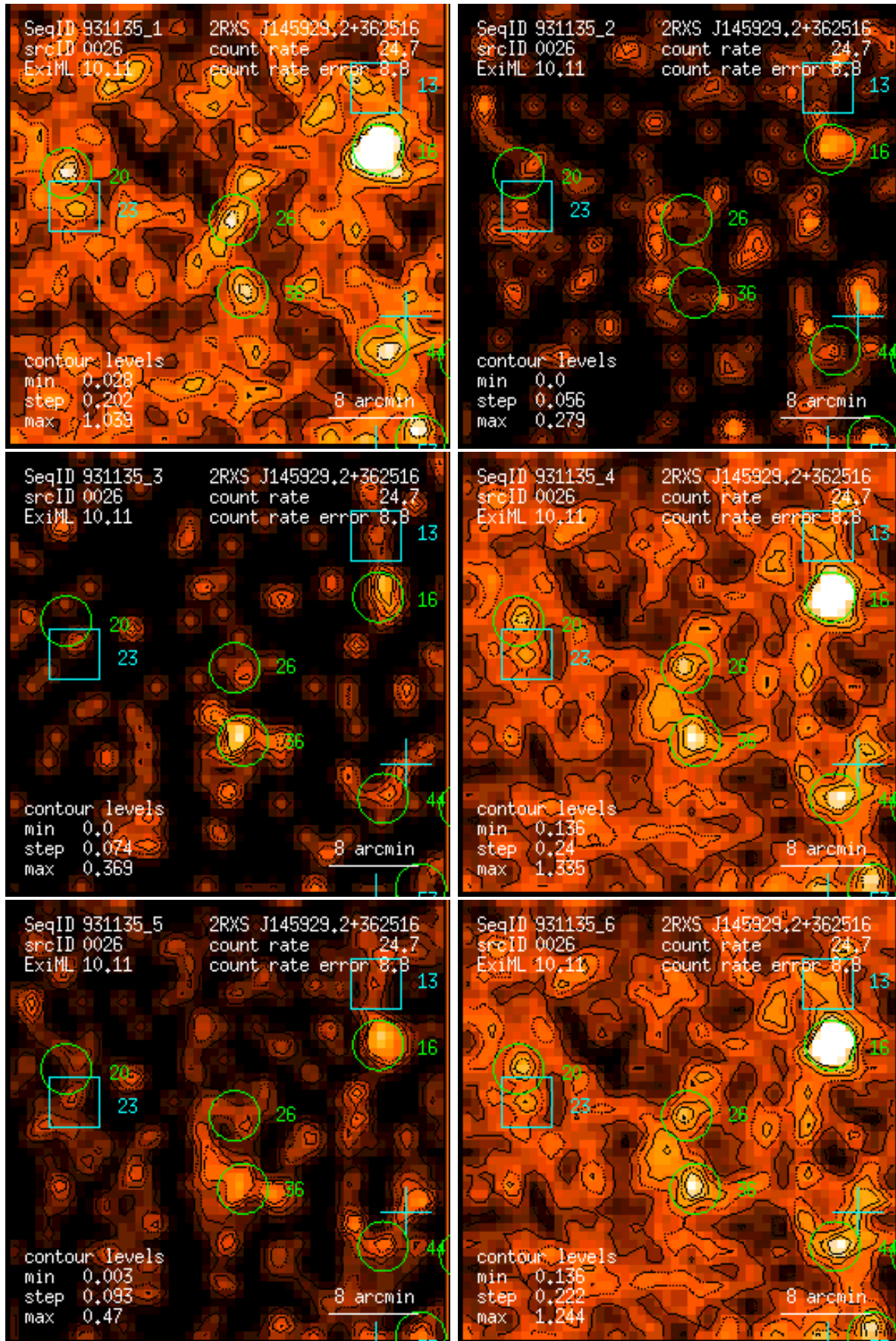
Figure 26: RASS 931135: detection 0026: band rate images, Gaussian filter: (1) PSPC channels 11 – 41, (2) 52 – 90, (3) 91 – 201, (4) 11 – 235, (5) 52 – 201, (6) 11 – 201. Broad band rates in counts/ks. Band rate contour levels in counts/ks/arcmin 2 .
