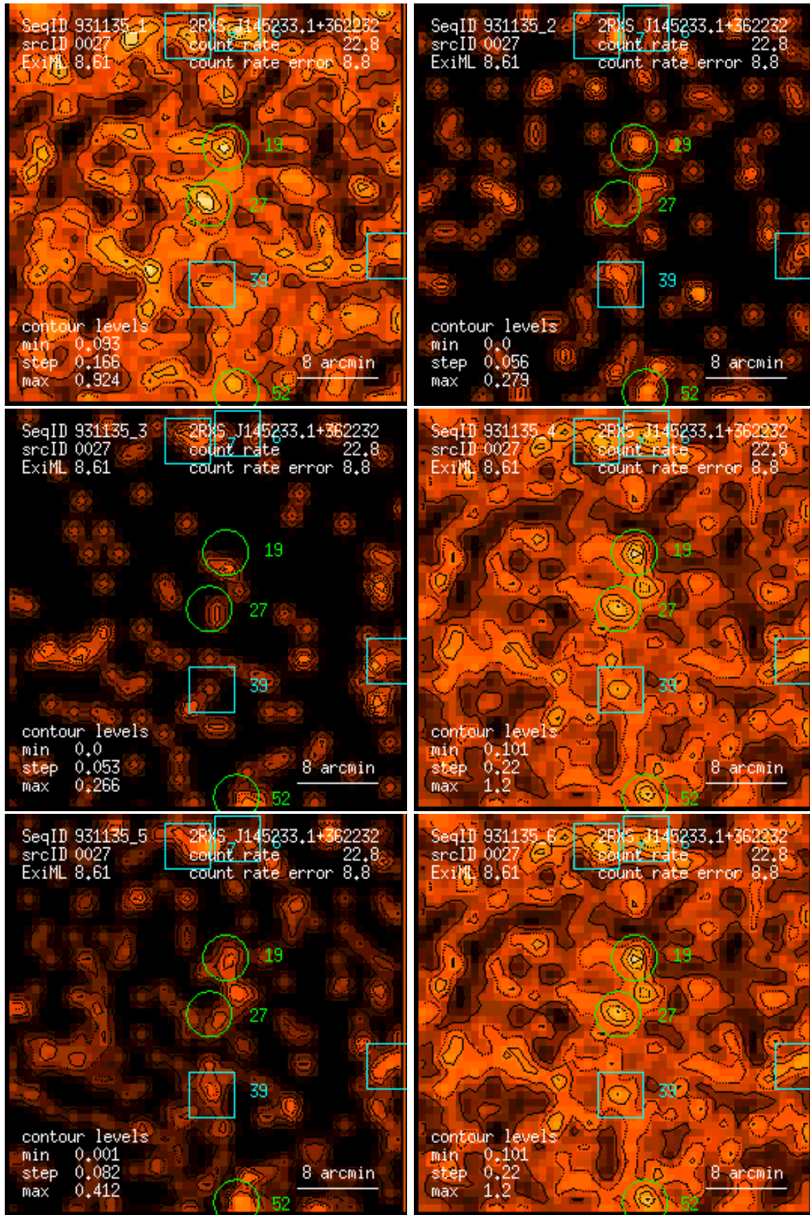
Figure 27: RASS 931135: detection 0027: band rate images, Gaussian filter: (1) PSPC channels 11 – 41, (2) 52 – 90, (3) 91 – 201, (4) 11 – 235, (5) 52 – 201, (6) 11 – 201. Broad band rates in counts/ks. Band rate contour levels in counts/ks/arcmin 2 .
