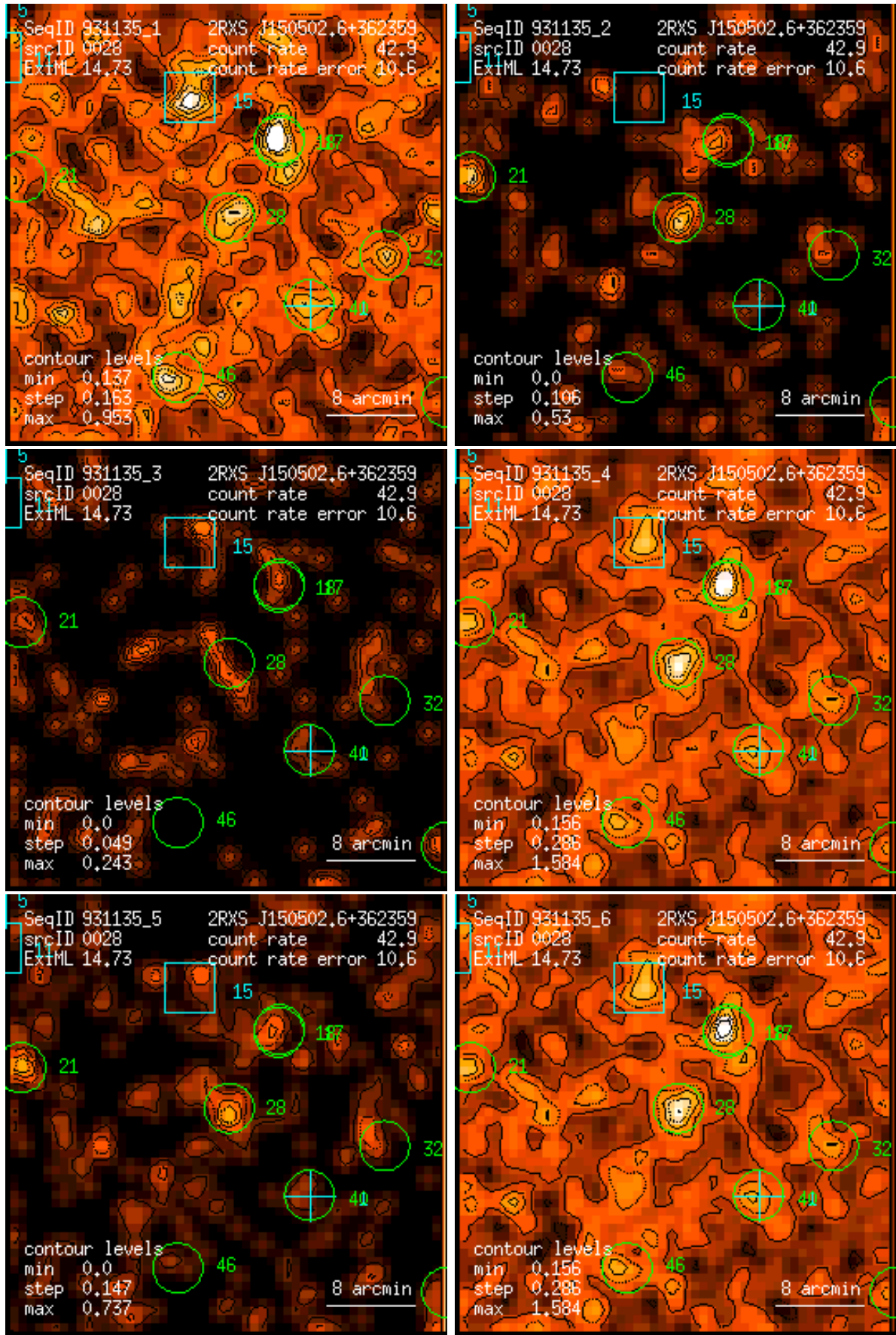
Figure 28: RASS 931135: detection 0028: band rate images, Gaussian filter: (1) PSPC channels 11 – 41, (2) 52 – 90, (3) 91 – 201, (4) 11 – 235, (5) 52 – 201, (6) 11 – 201. Broad band rates in counts/ks. Band rate contour levels in counts/ks/arcmin 2 .
