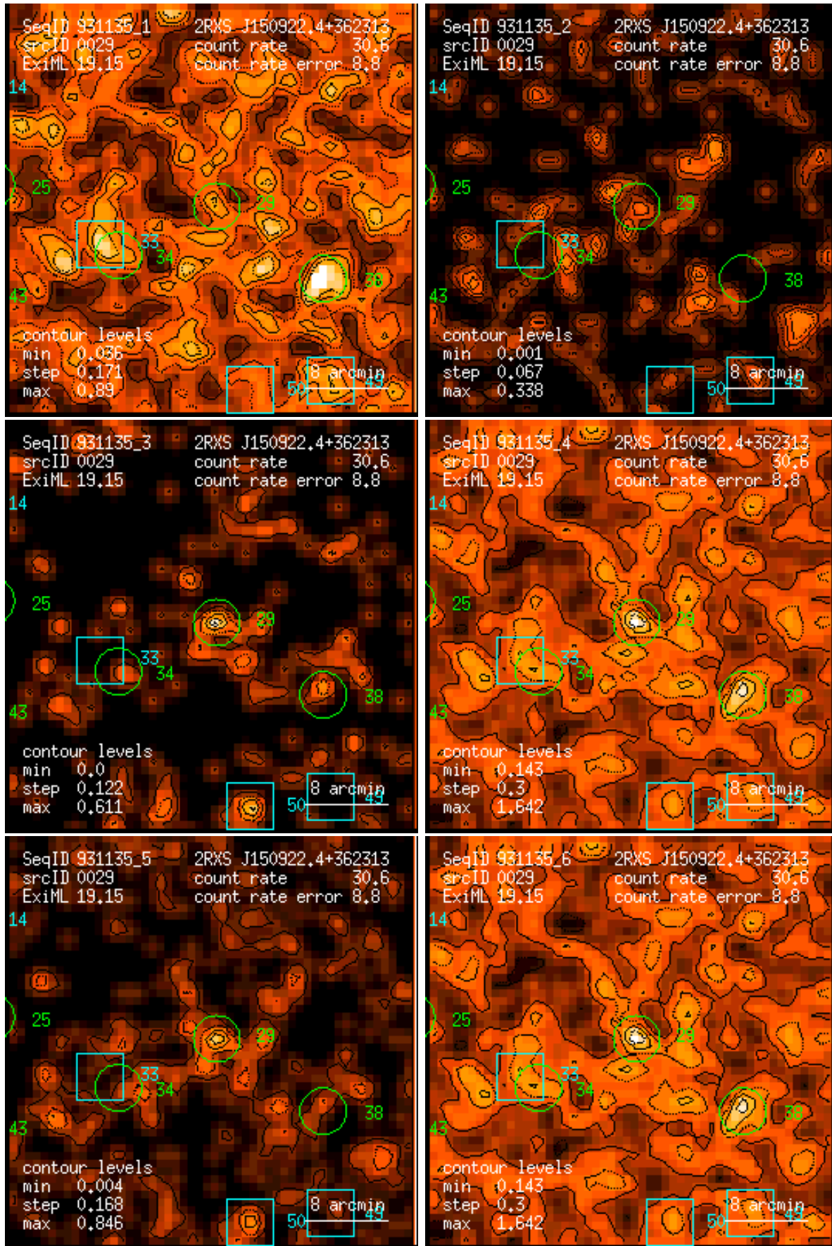
Figure 29: RASS 931135: detection 0029: band rate images, Gaussian filter: (1) PSPC channels 11 – 41, (2) 52 – 90, (3) 91 – 201, (4) 11 – 235, (5) 52 – 201, (6) 11 – 201. Broad band rates in counts/ks. Band rate contour levels in counts/ks/arcmin 2 .
