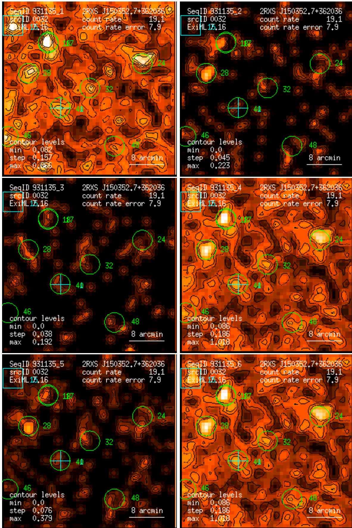
Figure 32: RASS 931135: detection 0032: band rate images, Gaussian filter: (1) PSPC channels 11 – 41, (2) 52 – 90, (3) 91 – 201, (4) 11 – 235, (5) 52 – 201, (6) 11 – 201. Broad band rates in counts/ks. Band rate contour levels in counts/ks/arcmin 2 .
