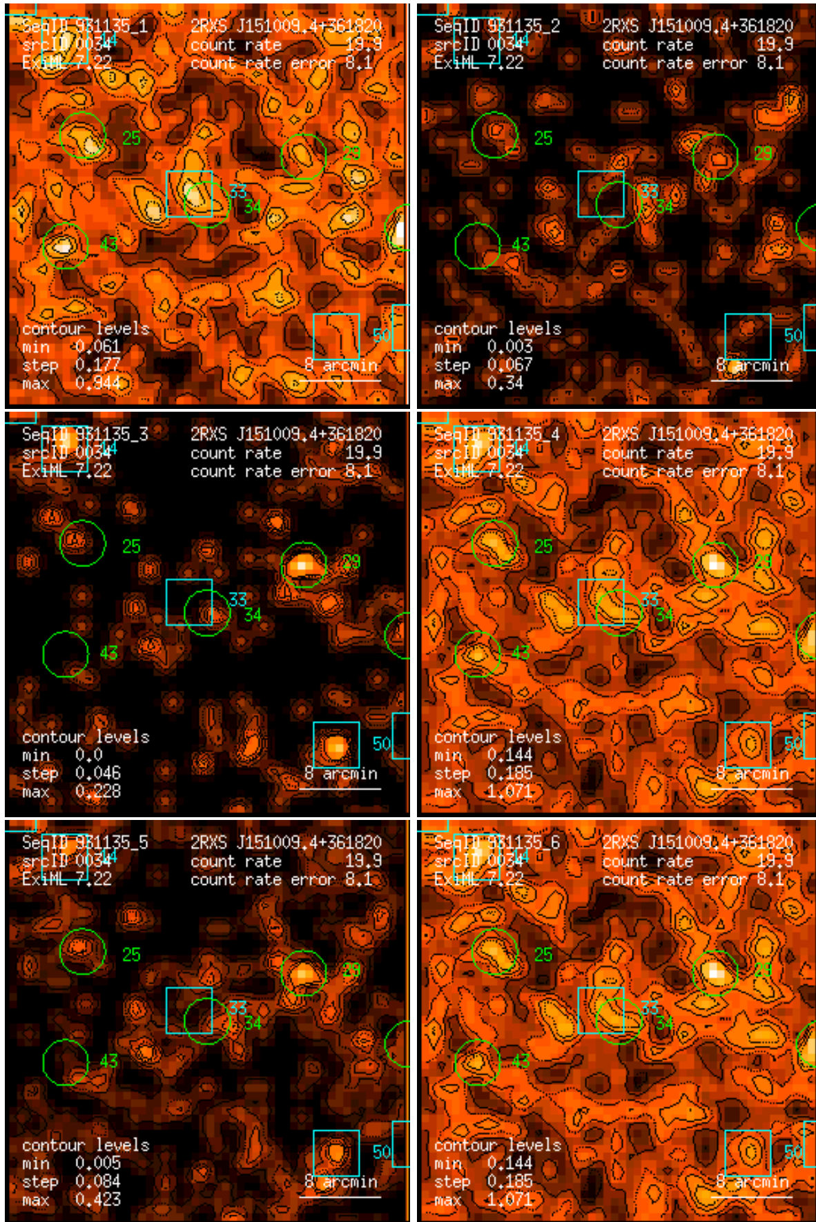
Figure 34: RASS 931135: detection 0034: band rate images, Gaussian filter: (1) PSPC channels 11 – 41, (2) 52 – 90, (3) 91 – 201, (4) 11 – 235, (5) 52 – 201, (6) 11 – 201. Broad band rates in counts/ks. Band rate contour levels in counts/ks/arcmin 2 .
