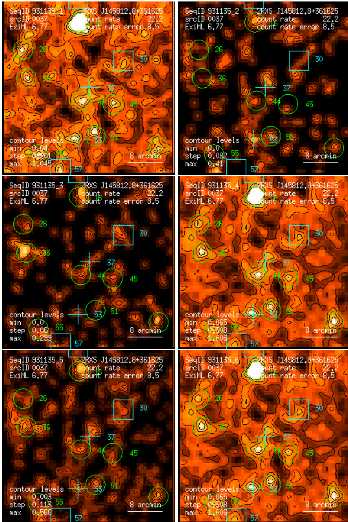
Figure 37: RASS 931135: detection 0037: band rate images, Gaussian filter: (1) PSPC channels 11 – 41, (2) 52 – 90, (3) 91 – 201, (4) 11 – 235, (5) 52 – 201, (6) 11 – 201. Broad band rates in counts/ks. Band rate contour levels in counts/ks/arcmin 2 .
