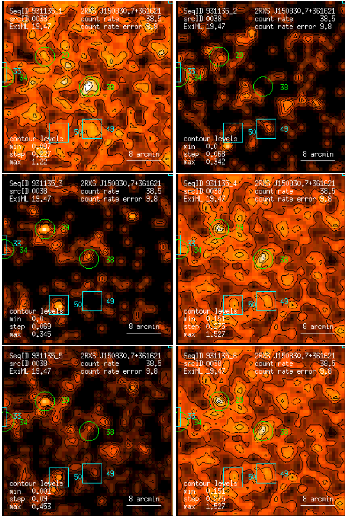
Figure 38: RASS 931135: detection 0038: band rate images, Gaussian filter: (1) PSPC channels 11 – 41, (2) 52 – 90, (3) 91 – 201, (4) 11 – 235, (5) 52 – 201, (6) 11 – 201. Broad band rates in counts/ks. Band rate contour levels in counts/ks/arcmin 2 .
