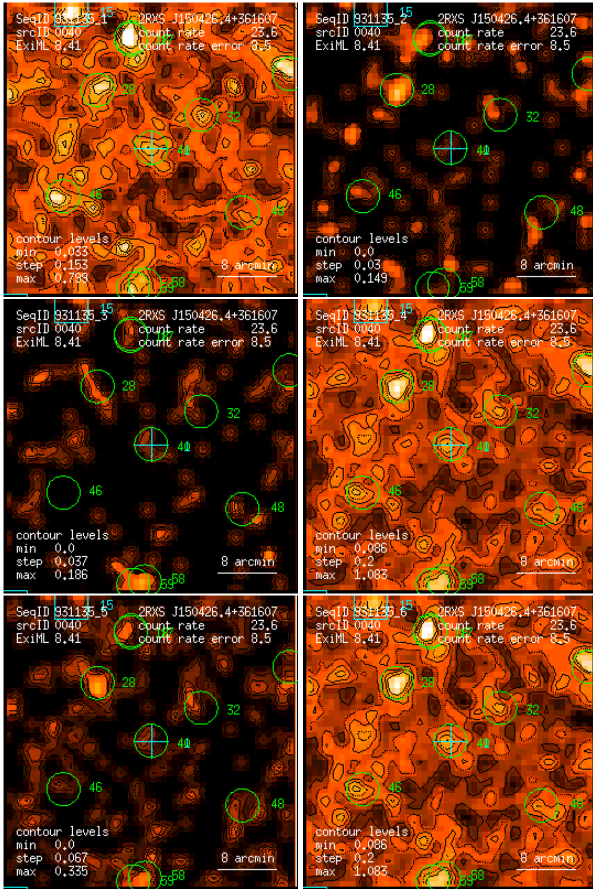
Figure 40: RASS 931135: detection 0040: band rate images, Gaussian filter: (1) PSPC channels 11 – 41, (2) 52 – 90, (3) 91 – 201, (4) 11 – 235, (5) 52 – 201, (6) 11 – 201. Broad band rates in counts/ks. Band rate contour levels in counts/ks/arcmin 2 .
