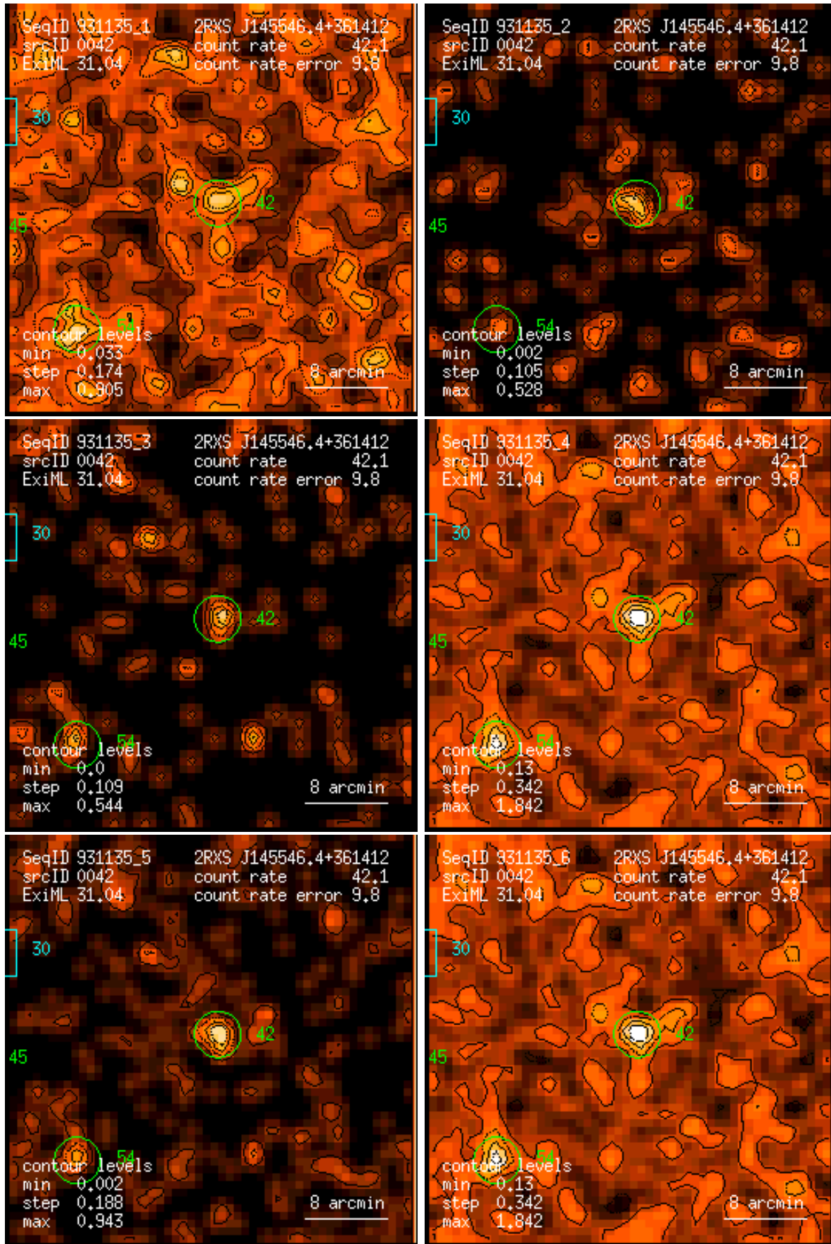
Figure 42: RASS 931135: detection 0042: band rate images, Gaussian filter: (1) PSPC channels 11 – 41, (2) 52 – 90, (3) 91 – 201, (4) 11 – 235, (5) 52 – 201, (6) 11 – 201. Broad band rates in counts/ks. Band rate contour levels in counts/ks/arcmin 2 .
