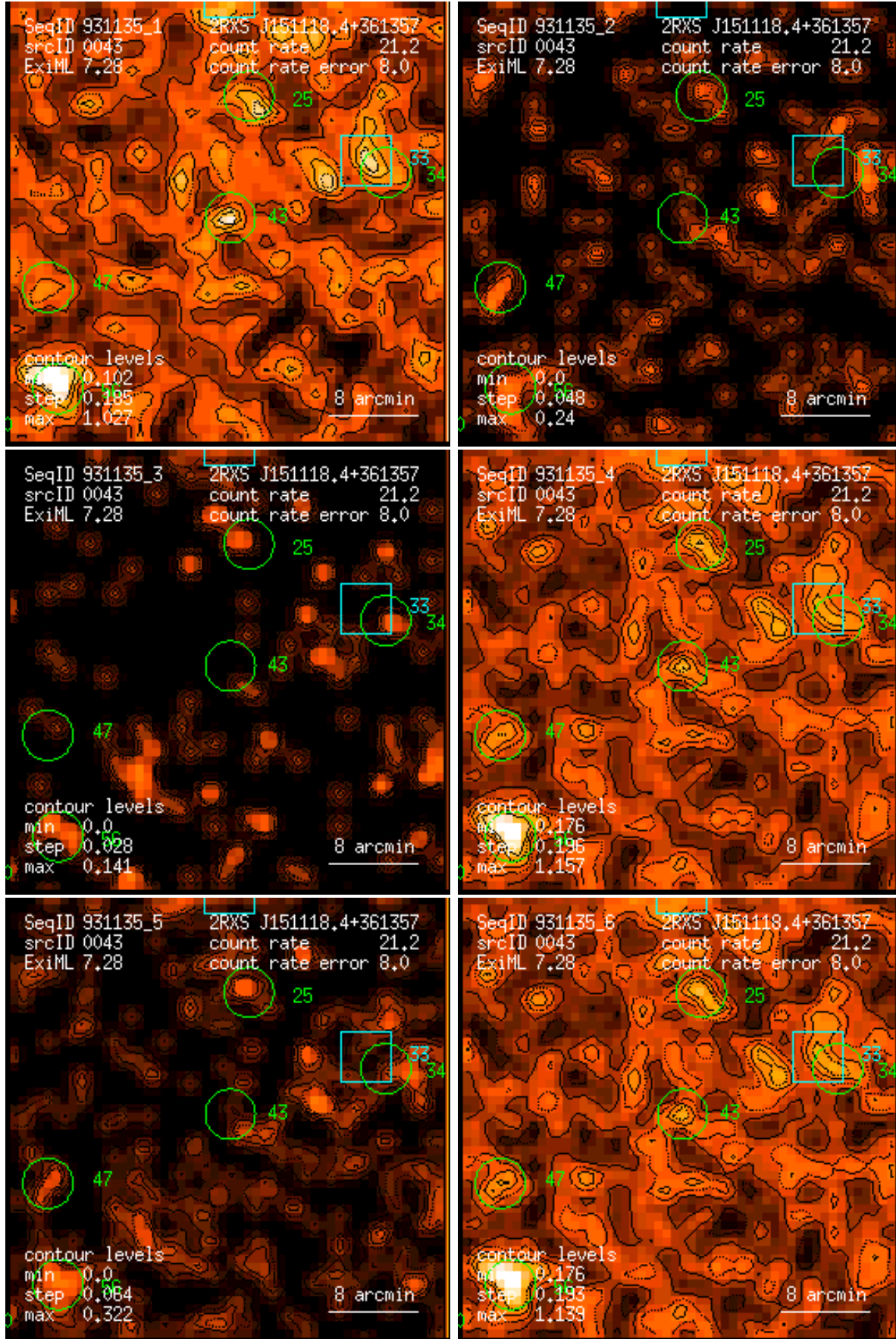
Figure 43: RASS 931135: detection 0043: band rate images, Gaussian filter: (1) PSPC channels 11 – 41, (2) 52 – 90, (3) 91 – 201, (4) 11 – 235, (5) 52 – 201, (6) 11 – 201. Broad band rates in counts/ks. Band rate contour levels in counts/ks/arcmin 2 .
