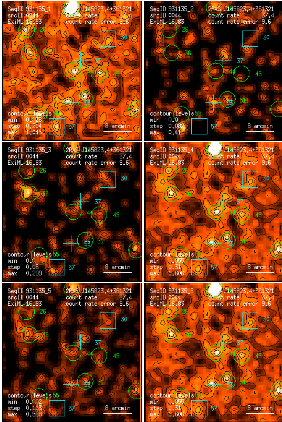
Figure 44: RASS 931135: detection 0044: band rate images, Gaussian filter: (1) PSPC channels 11 – 41, (2) 52 – 90, (3) 91 – 201, (4) 11 – 235, (5) 52 – 201, (6) 11 – 201. Broad band rates in counts/ks. Band rate contour levels in counts/ks/arcmin 2 .
