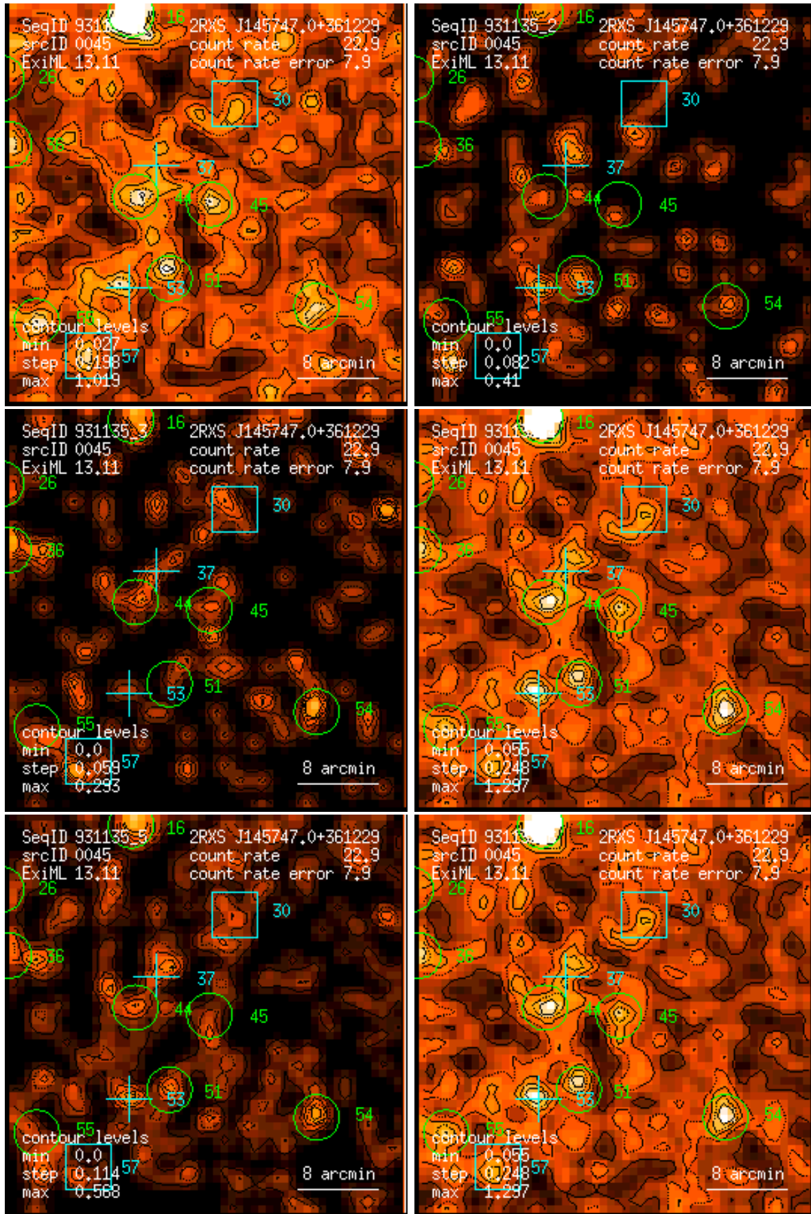
Figure 45: RASS 931135: detection 0045: band rate images, Gaussian filter: (1) PSPC channels 11 – 41, (2) 52 – 90, (3) 91 – 201, (4) 11 – 235, (5) 52 – 201, (6) 11 – 201. Broad band rates in counts/ks. Band rate contour levels in counts/ks/arcmin 2 .
