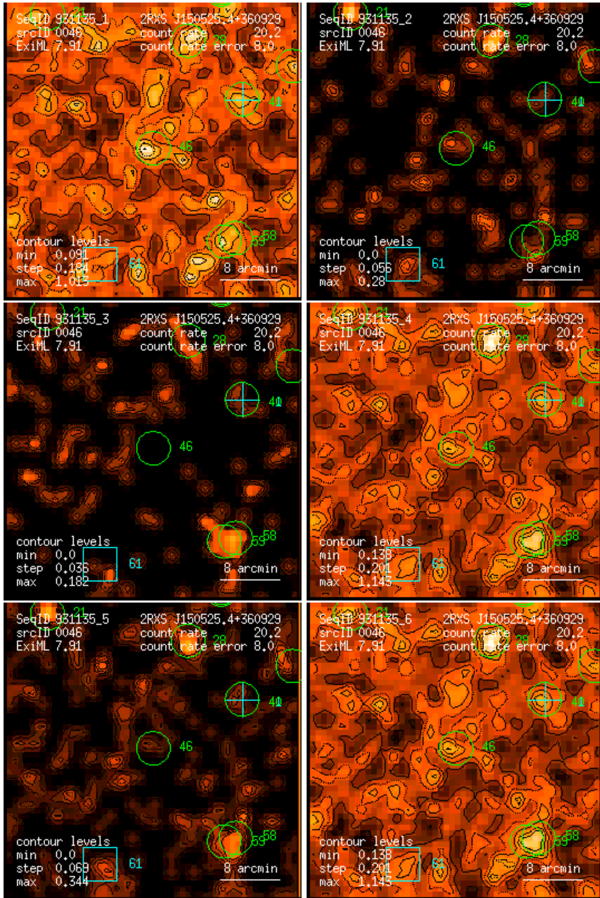
Figure 46: RASS 931135: detection 0046: band rate images, Gaussian filter: (1) PSPC channels 11 – 41, (2) 52 – 90, (3) 91 – 201, (4) 11 – 235, (5) 52 – 201, (6) 11 – 201. Broad band rates in counts/ks. Band rate contour levels in counts/ks/arcmin 2 .
