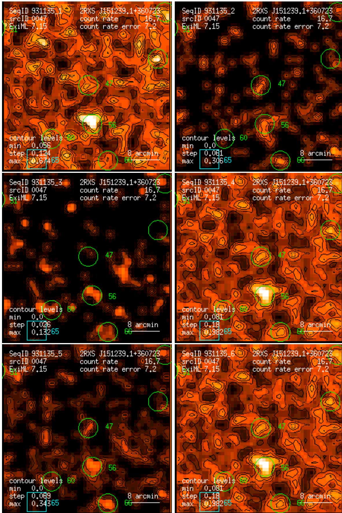
Figure 47: RASS 931135: detection 0047: band rate images, Gaussian filter: (1) PSPC channels 11 – 41, (2) 52 – 90, (3) 91 – 201, (4) 11 – 235, (5) 52 – 201, (6) 11 – 201. Broad band rates in counts/ks. Band rate contour levels in counts/ks/arcmin 2 .
