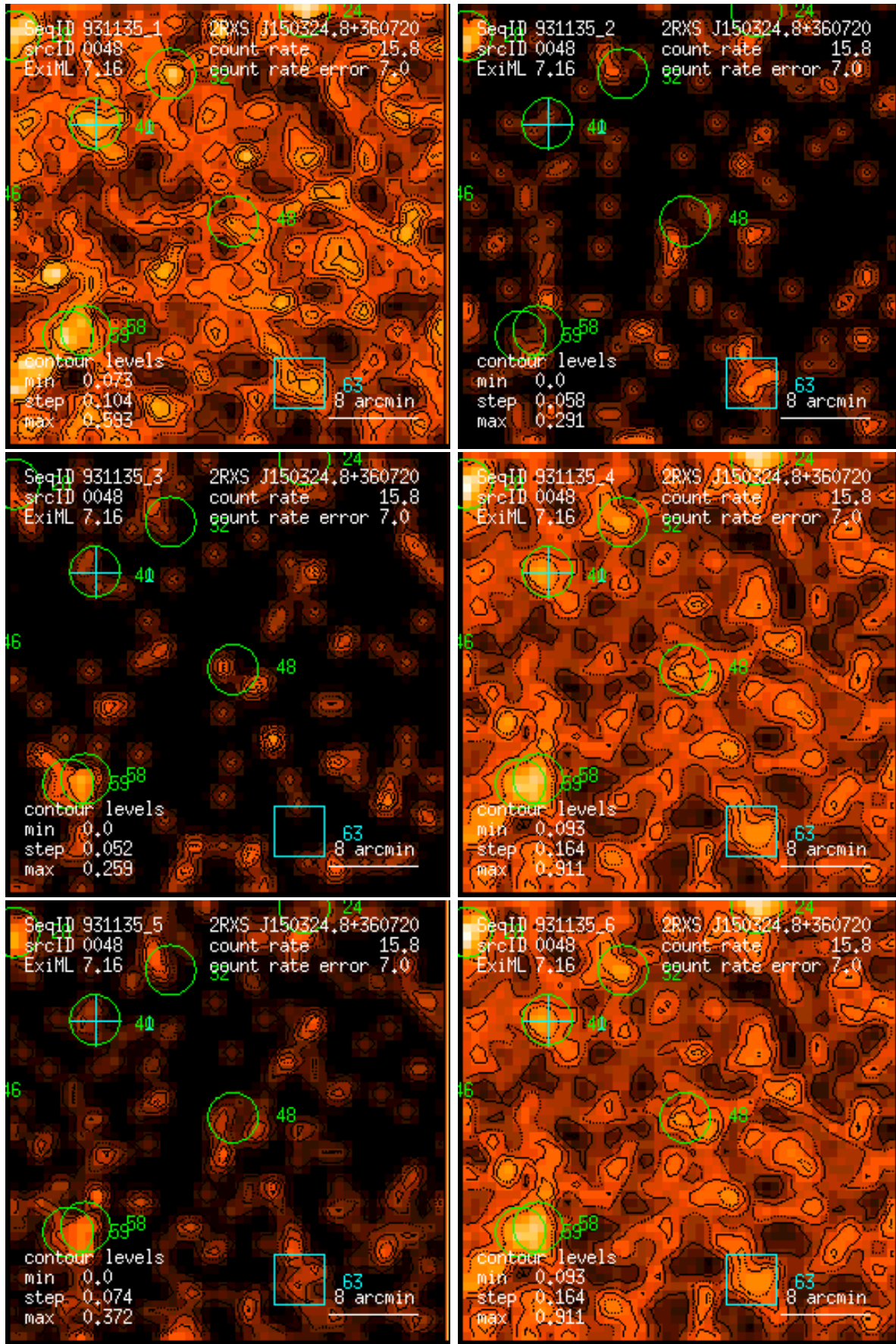
Figure 48: RASS 931135: detection 0048: band rate images, Gaussian filter: (1) PSPC channels 11 – 41, (2) 52 – 90, (3) 91 – 201, (4) 11 – 235, (5) 52 – 201, (6) 11 – 201. Broad band rates in counts/ks. Band rate contour levels in counts/ks/arcmin 2 .
