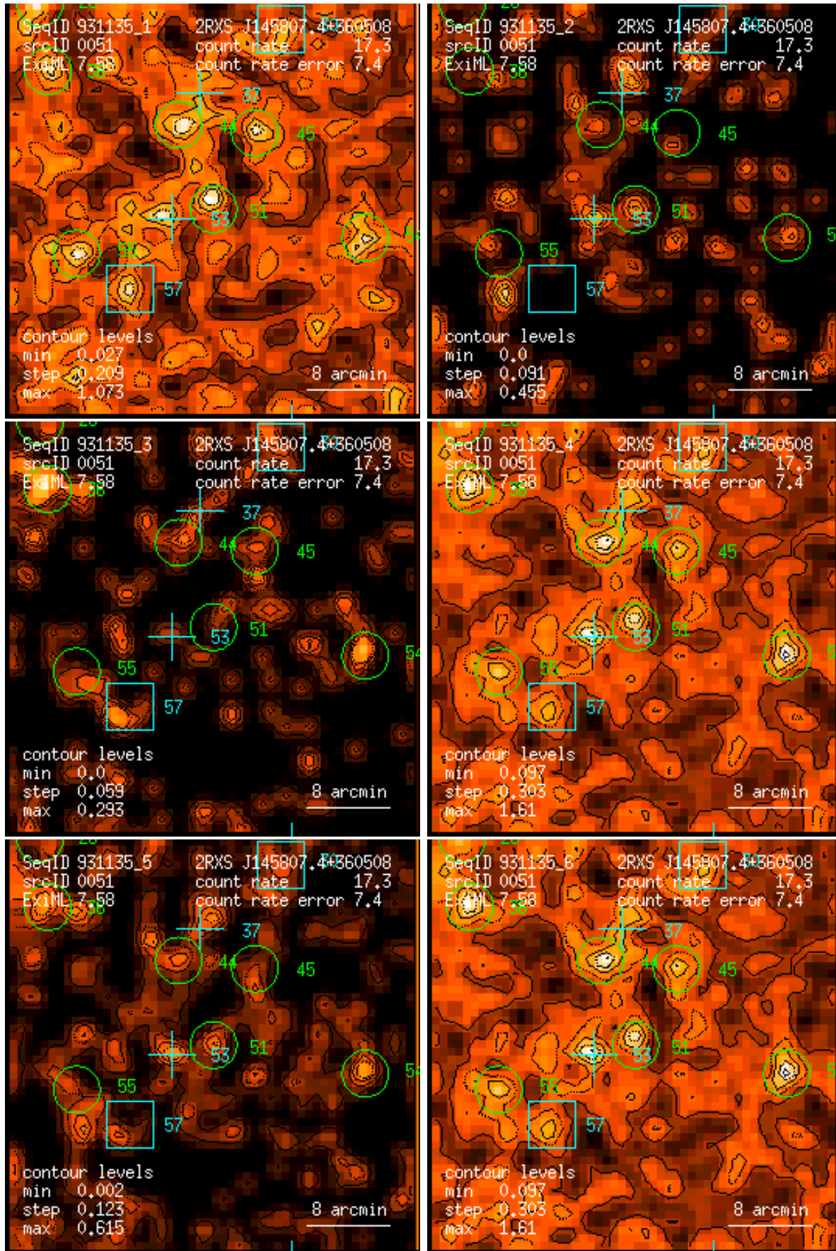
Figure 51: RASS 931135: detection 0051: band rate images, Gaussian filter: (1) PSPC channels 11 – 41, (2) 52 – 90, (3) 91 – 201, (4) 11 – 235, (5) 52 – 201, (6) 11 – 201. Broad band rates in counts/ks. Band rate contour levels in counts/ks/arcmin 2 .
