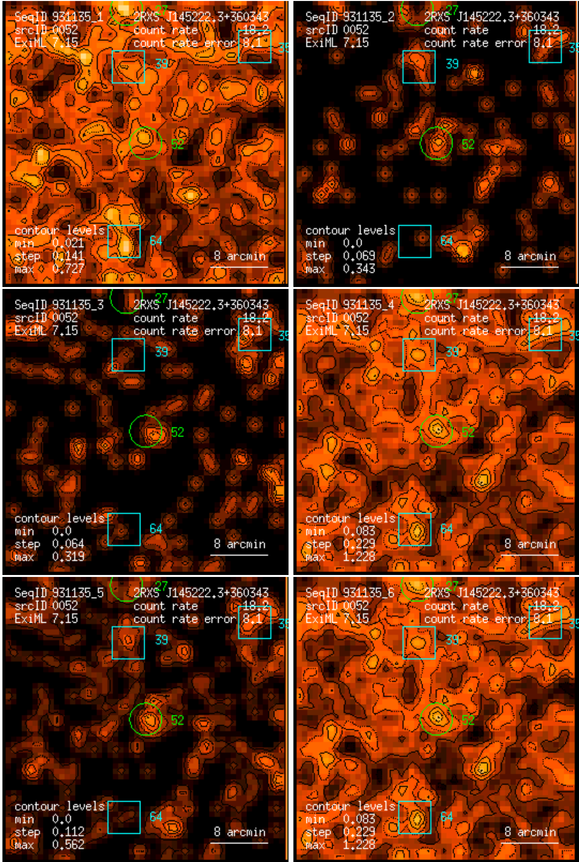
Figure 52: RASS 931135: detection 0052: band rate images, Gaussian filter: (1) PSPC channels 11 – 41, (2) 52 – 90, (3) 91 – 201, (4) 11 – 235, (5) 52 – 201, (6) 11 – 201. Broad band rates in counts/ks. Band rate contour levels in counts/ks/arcmin 2 .
