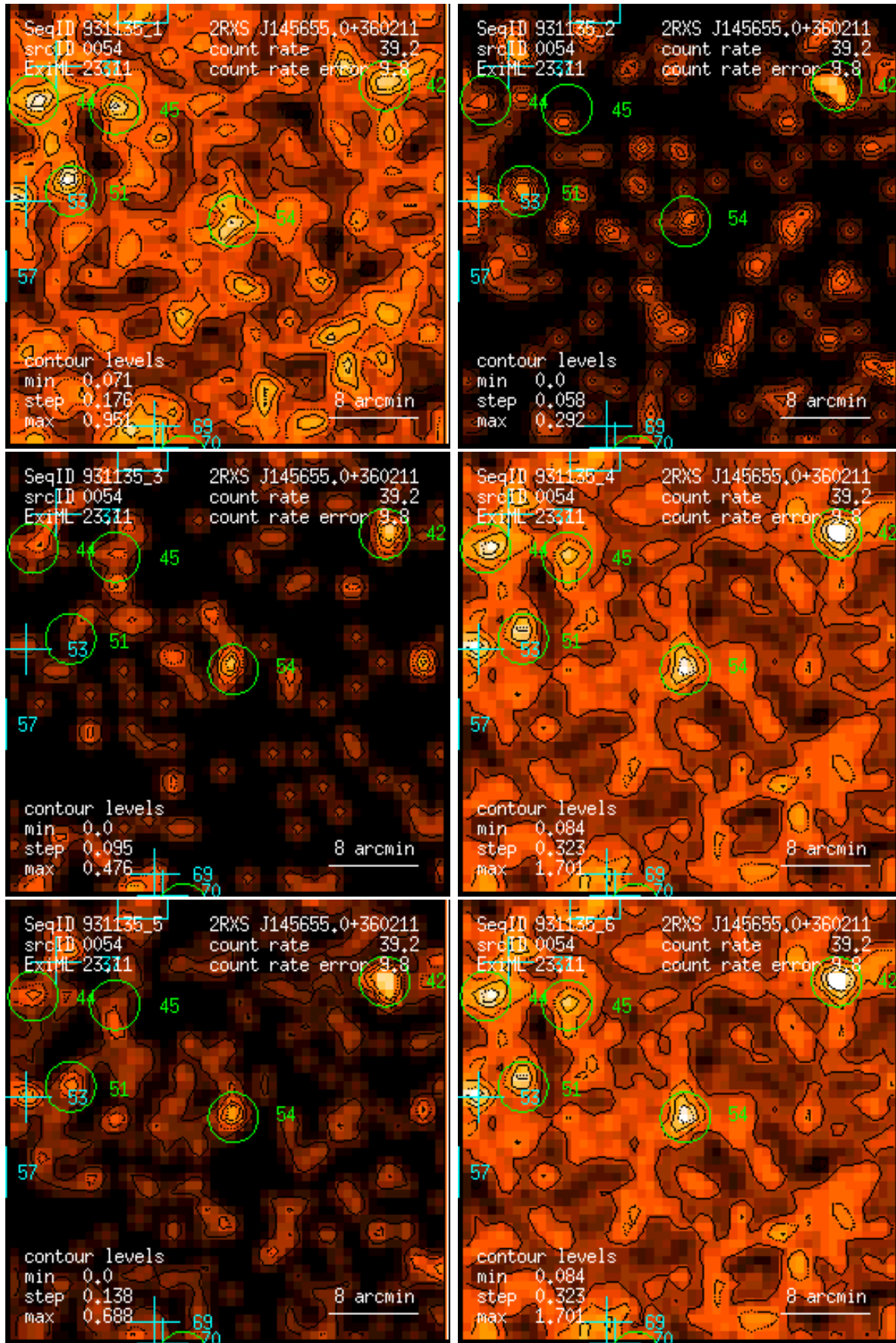
Figure 54: RASS 931135: detection 0054: band rate images, Gaussian filter: (1) PSPC channels 11 – 41, (2) 52 – 90, (3) 91 – 201, (4) 11 – 235, (5) 52 – 201, (6) 11 – 201. Broad band rates in counts/ks. Band rate contour levels in counts/ks/arcmin 2 .
