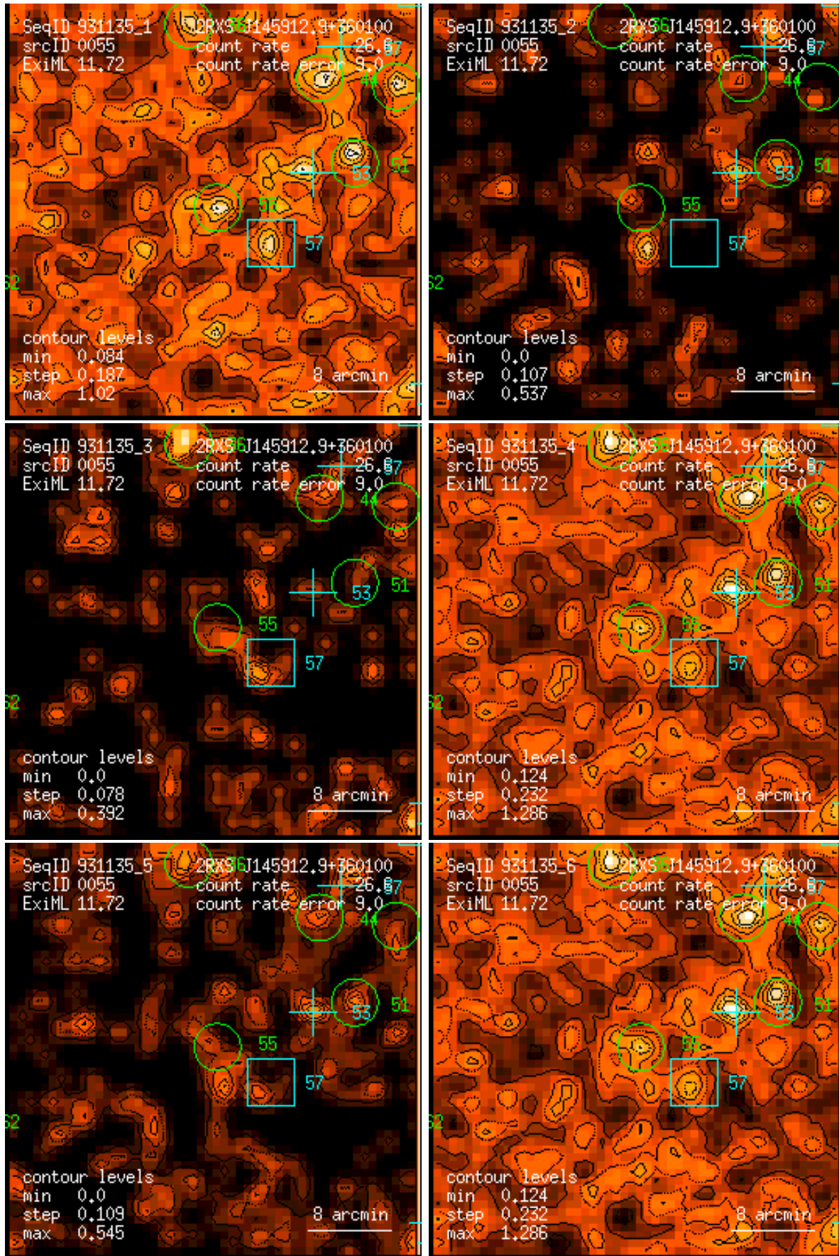
Figure 55: RASS 931135: detection 0055: band rate images, Gaussian filter: (1) PSPC channels 11 – 41, (2) 52 – 90, (3) 91 – 201, (4) 11 – 235, (5) 52 – 201, (6) 11 – 201. Broad band rates in counts/ks. Band rate contour levels in counts/ks/arcmin 2 .
