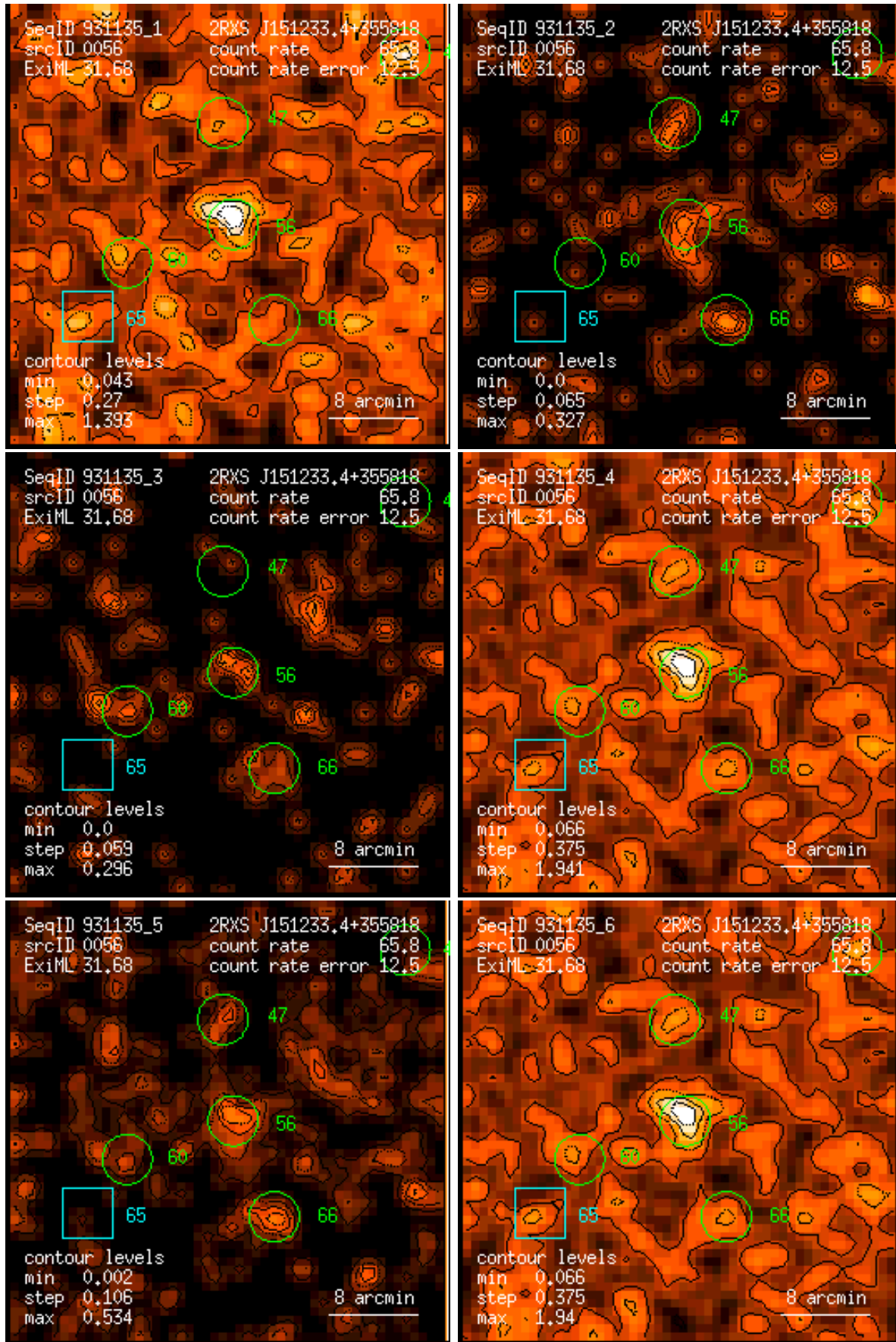
Figure 56: RASS 931135: detection 0056: band rate images, Gaussian filter: (1) PSPC channels 11 – 41, (2) 52 – 90, (3) 91 – 201, (4) 11 – 235, (5) 52 – 201, (6) 11 – 201. Broad band rates in counts/ks. Band rate contour levels in counts/ks/arcmin 2 .
