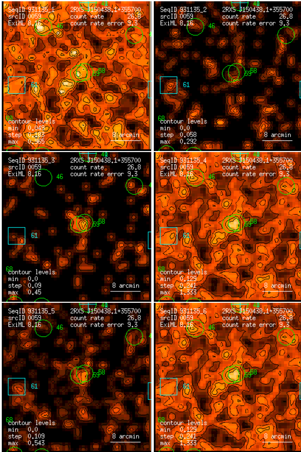
Figure 59: RASS 931135: detection 0059: band rate images, Gaussian filter: (1) PSPC channels 11 – 41, (2) 52 – 90, (3) 91 – 201, (4) 11 – 235, (5) 52 – 201, (6) 11 – 201. Broad band rates in counts/ks. Band rate contour levels in counts/ks/arcmin 2 .
