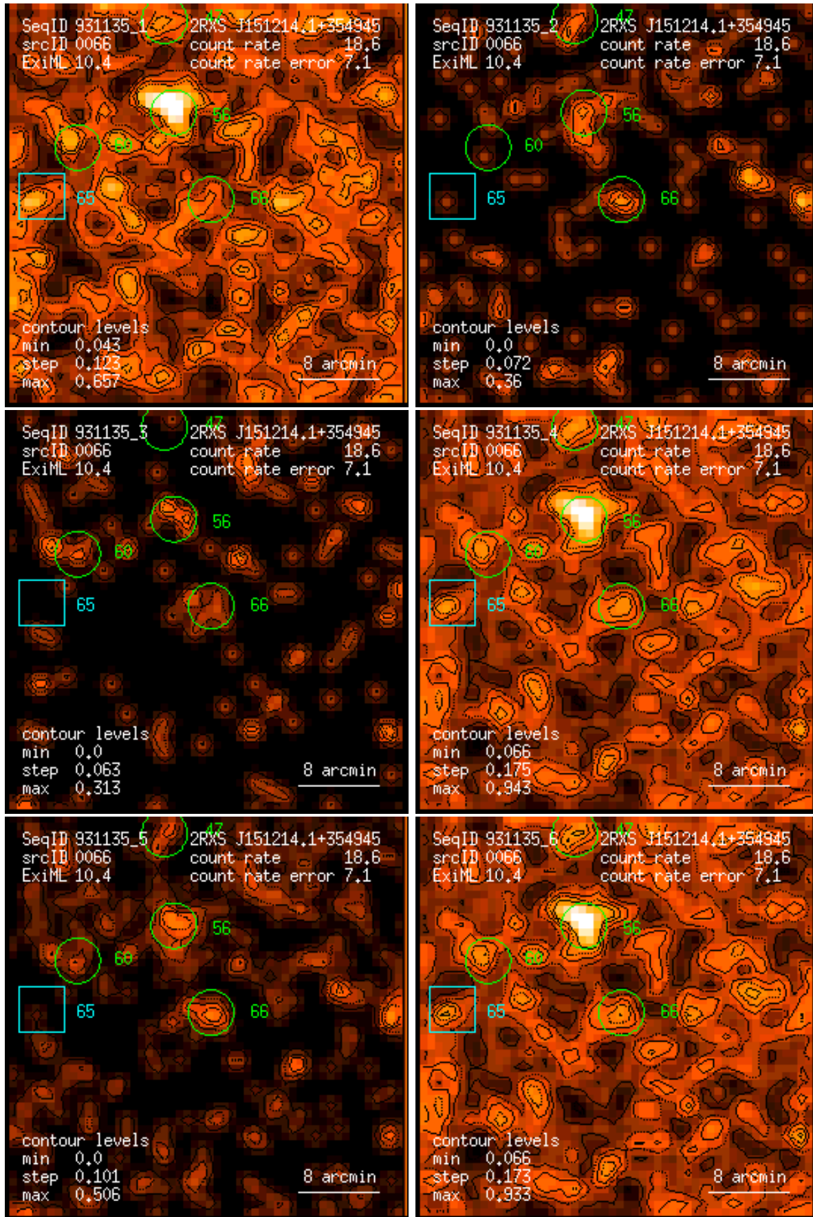
Figure 66: RASS 931135: detection 0066: band rate images, Gaussian filter: (1) PSPC channels 11 – 41, (2) 52 – 90, (3) 91 – 201, (4) 11 – 235, (5) 52 – 201, (6) 11 – 201. Broad band rates in counts/ks. Band rate contour levels in counts/ks/arcmin 2 .
