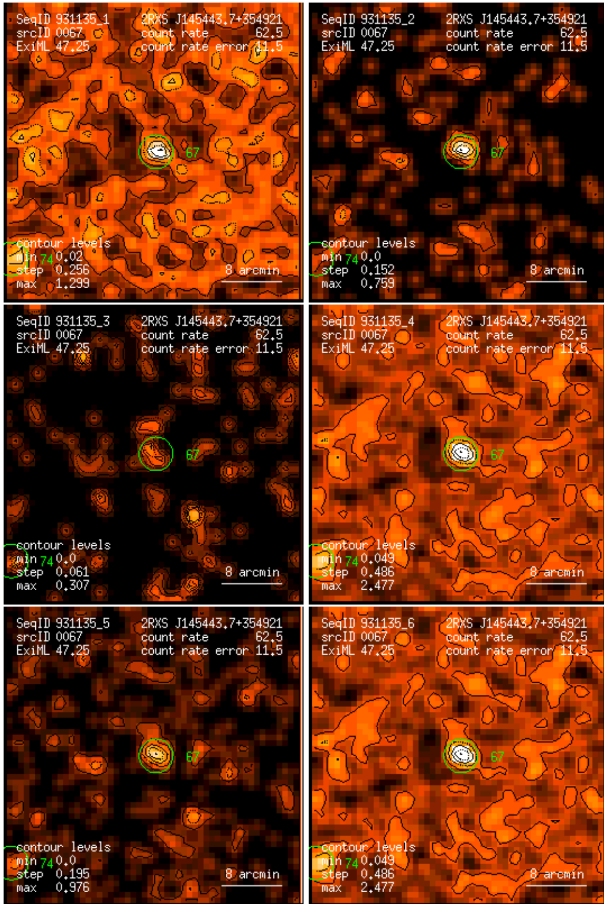
Figure 67: RASS 931135: detection 0067: band rate images, Gaussian filter: (1) PSPC channels 11 – 41, (2) 52 – 90, (3) 91 – 201, (4) 11 – 235, (5) 52 – 201, (6) 11 – 201. Broad band rates in counts/ks. Band rate contour levels in counts/ks/arcmin 2 .
