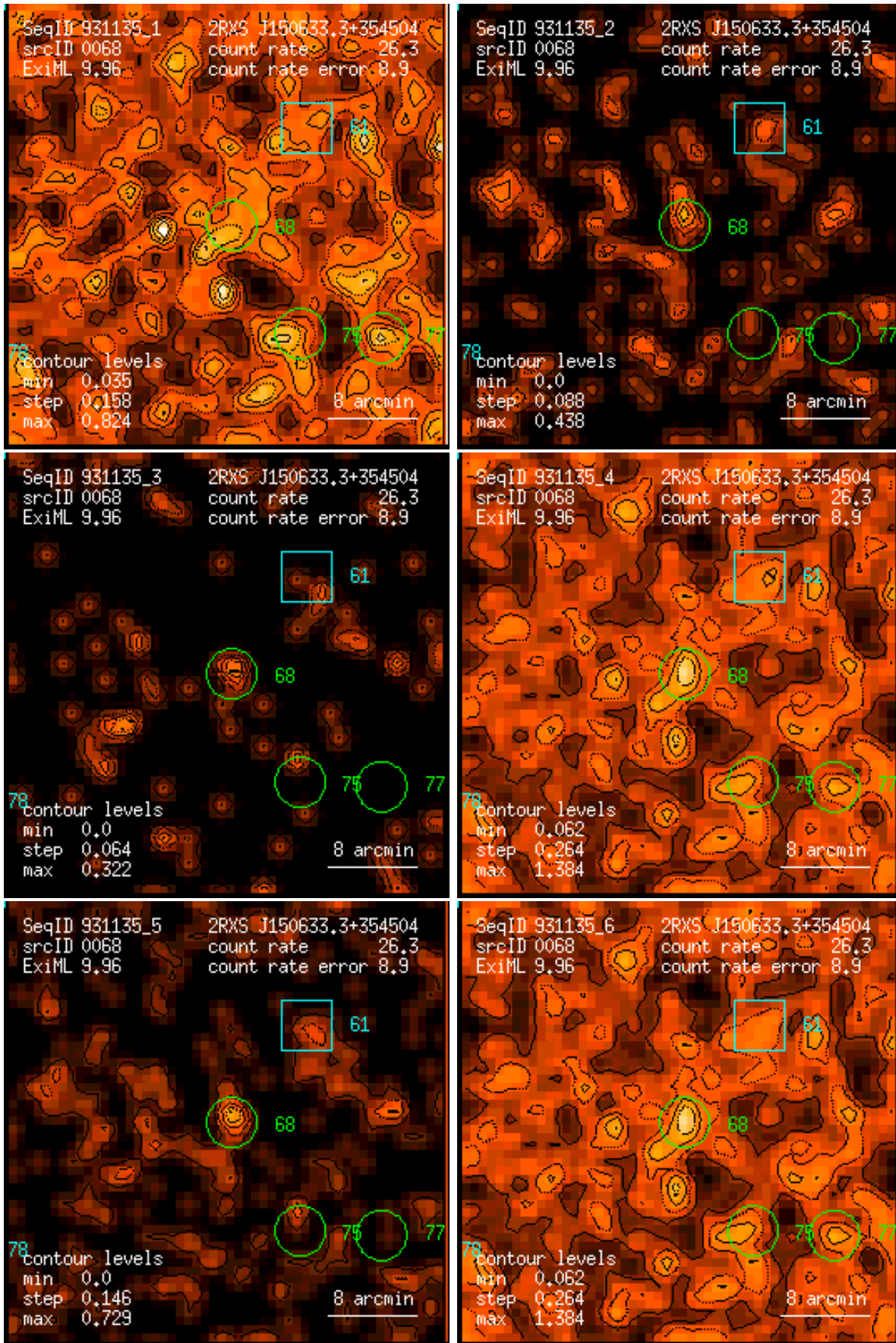
Figure 68: RASS 931135: detection 0068: band rate images, Gaussian filter: (1) PSPC channels 11 – 41, (2) 52 – 90, (3) 91 – 201, (4) 11 – 235, (5) 52 – 201, (6) 11 – 201. Broad band rates in counts/ks. Band rate contour levels in counts/ks/arcmin 2 .
