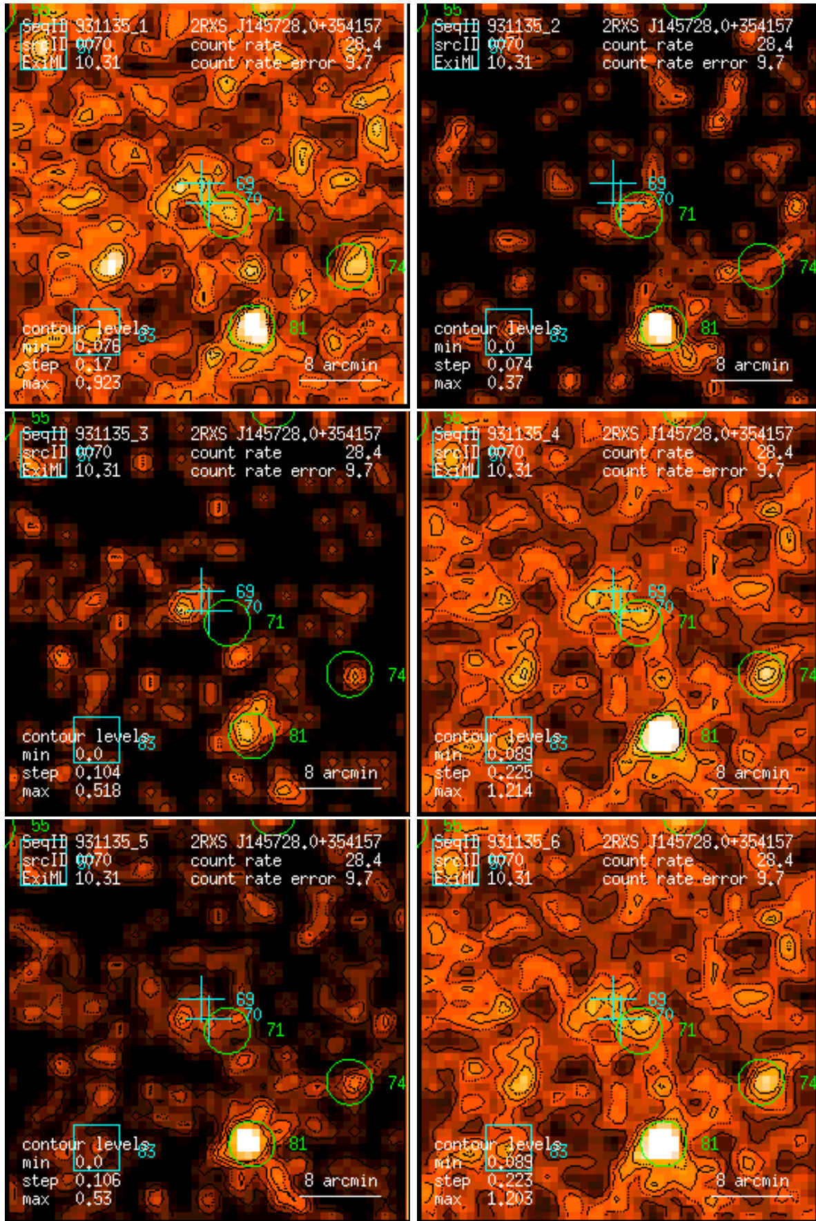
Figure 70: RASS 931135: detection 0070: band rate images, Gaussian filter: (1) PSPC channels 11 – 41, (2) 52 – 90, (3) 91 – 201, (4) 11 – 235, (5) 52 – 201, (6) 11 – 201. Broad band rates in counts/ks. Band rate contour levels in counts/ks/arcmin 2 .
