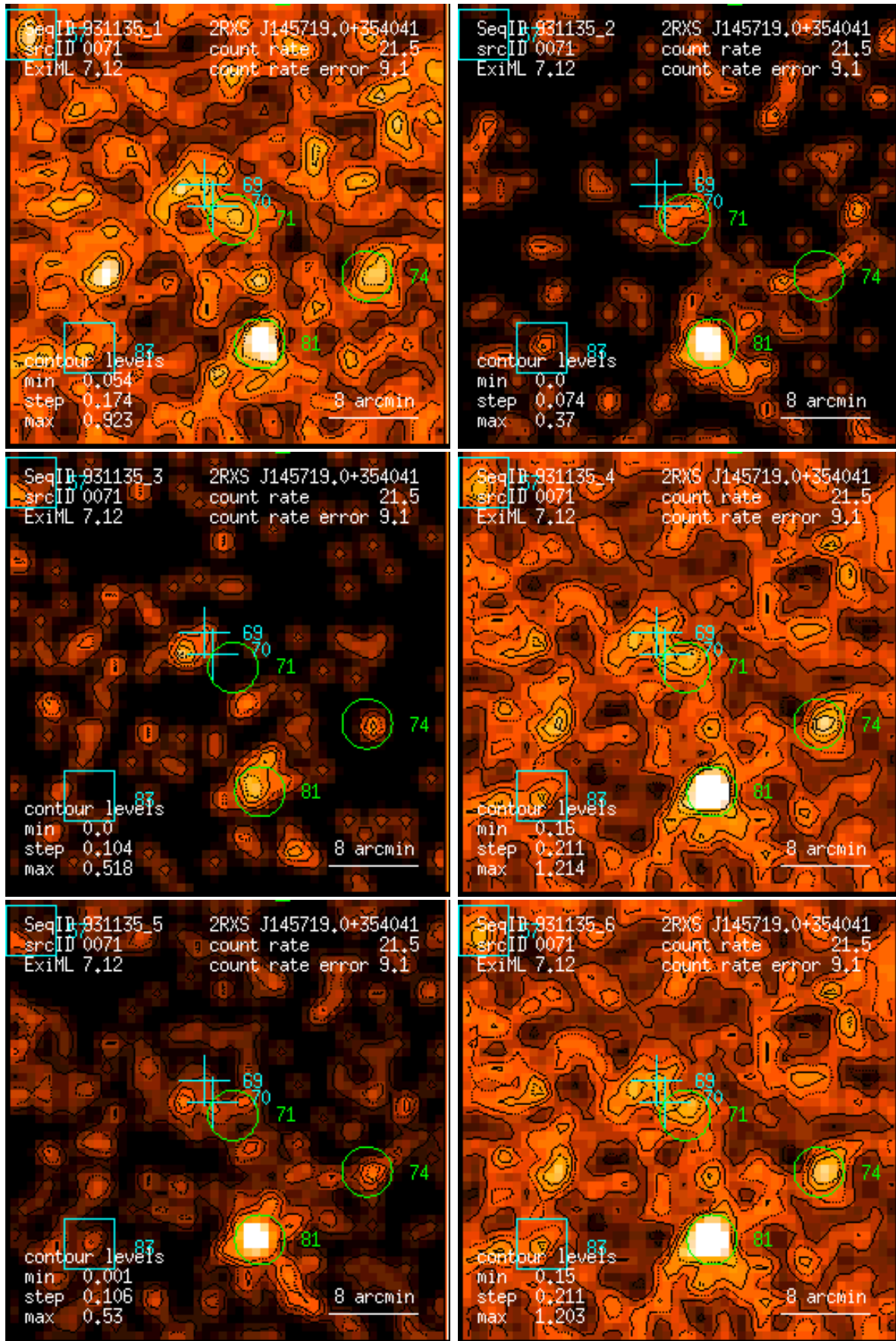
Figure 71: RASS 931135: detection 0071: band rate images, Gaussian filter: (1) PSPC channels 11 – 41, (2) 52 – 90, (3) 91 – 201, (4) 11 – 235, (5) 52 – 201, (6) 11 – 201. Broad band rates in counts/ks. Band rate contour levels in counts/ks/arcmin 2 .
