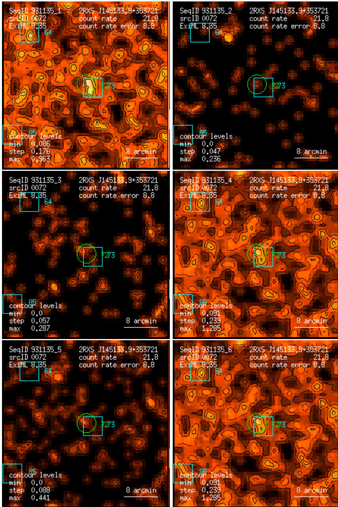
Figure 72: RASS 931135: detection 0072: band rate images, Gaussian filter: (1) PSPC channels 11 – 41, (2) 52 – 90, (3) 91 – 201, (4) 11 – 235, (5) 52 – 201, (6) 11 – 201. Broad band rates in counts/ks. Band rate contour levels in counts/ks/arcmin 2 .
