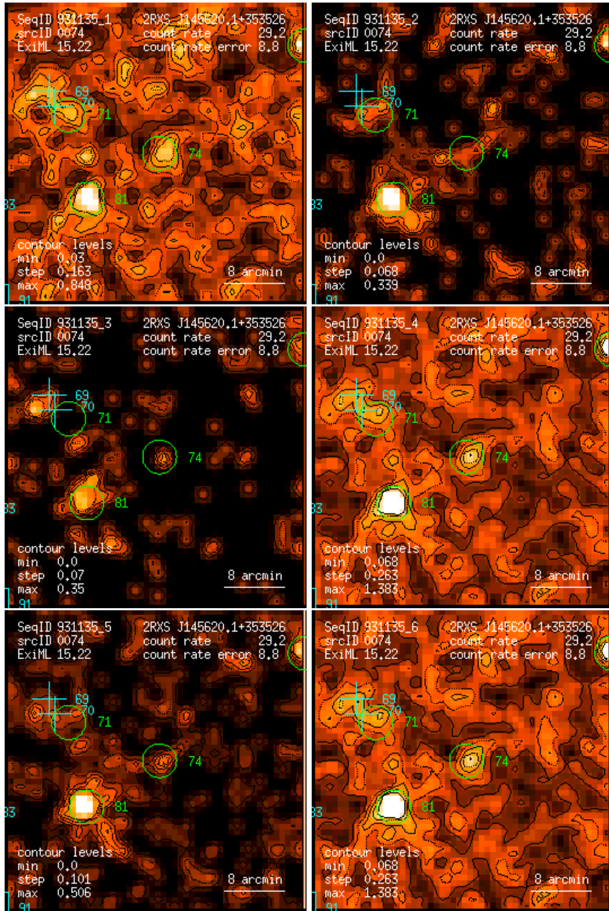
Figure 74: RASS 931135: detection 0074: band rate images, Gaussian filter: (1) PSPC channels 11 – 41, (2) 52 – 90, (3) 91 – 201, (4) 11 – 235, (5) 52 – 201, (6) 11 – 201. Broad band rates in counts/ks. Band rate contour levels in counts/ks/arcmin 2 .
