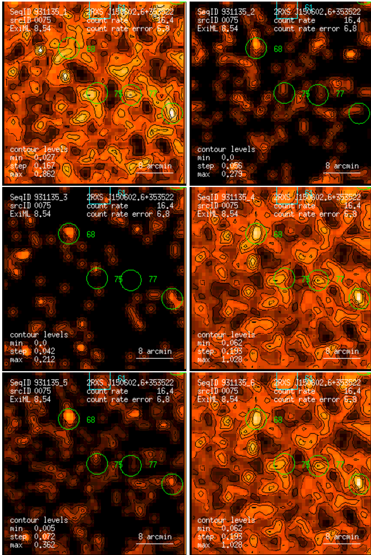
Figure 75: RASS 931135: detection 0075: band rate images, Gaussian filter: (1) PSPC channels 11 – 41, (2) 52 – 90, (3) 91 – 201, (4) 11 – 235, (5) 52 – 201, (6) 11 – 201. Broad band rates in counts/ks. Band rate contour levels in counts/ks/arcmin 2 .
