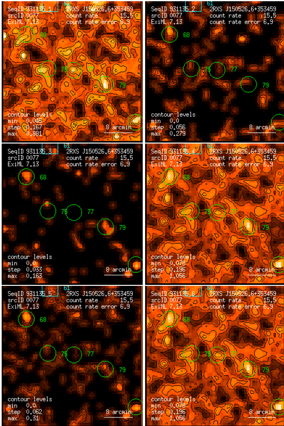
Figure 77: RASS 931135: detection 0077: band rate images, Gaussian filter: (1) PSPC channels 11 – 41, (2) 52 – 90, (3) 91 – 201, (4) 11 – 235, (5) 52 – 201, (6) 11 – 201. Broad band rates in counts/ks. Band rate contour levels in counts/ks/arcmin 2 .
