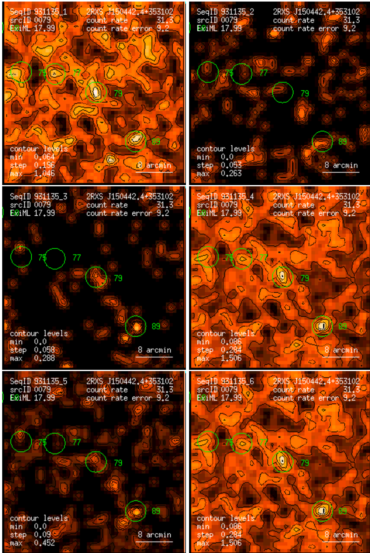
Figure 79: RASS 931135: detection 0079: band rate images, Gaussian filter: (1) PSPC channels 11 – 41, (2) 52 – 90, (3) 91 – 201, (4) 11 – 235, (5) 52 – 201, (6) 11 – 201. Broad band rates in counts/ks. Band rate contour levels in counts/ks/arcmin 2 .
