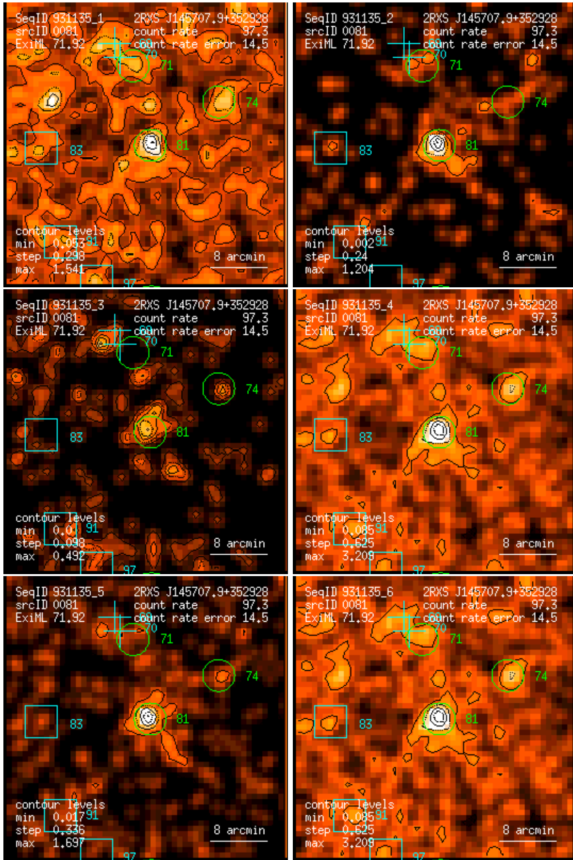
Figure 81: RASS 931135: detection 0081: band rate images, Gaussian filter: (1) PSPC channels 11 – 41, (2) 52 – 90, (3) 91 – 201, (4) 11 – 235, (5) 52 – 201, (6) 11 – 201. Broad band rates in counts/ks. Band rate contour levels in counts/ks/arcmin 2 .
