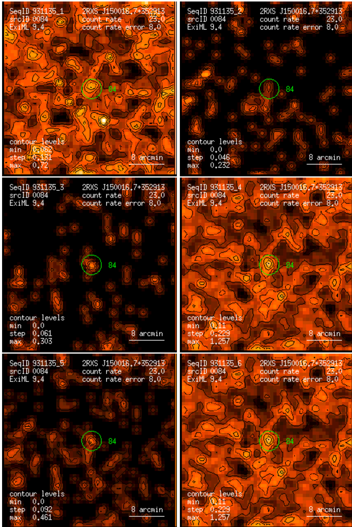
Figure 84: RASS 931135: detection 0084: band rate images, Gaussian filter: (1) PSPC channels 11 – 41, (2) 52 – 90, (3) 91 – 201, (4) 11 – 235, (5) 52 – 201, (6) 11 – 201. Broad band rates in counts/ks. Band rate contour levels in counts/ks/arcmin 2 .
