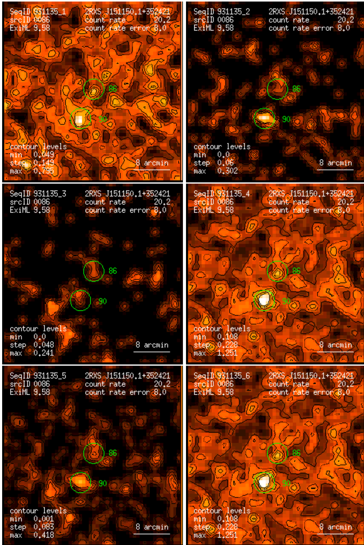
Figure 86: RASS 931135: detection 0086: band rate images, Gaussian filter: (1) PSPC channels 11 – 41, (2) 52 – 90, (3) 91 – 201, (4) 11 – 235, (5) 52 – 201, (6) 11 – 201. Broad band rates in counts/ks. Band rate contour levels in counts/ks/arcmin 2 .
