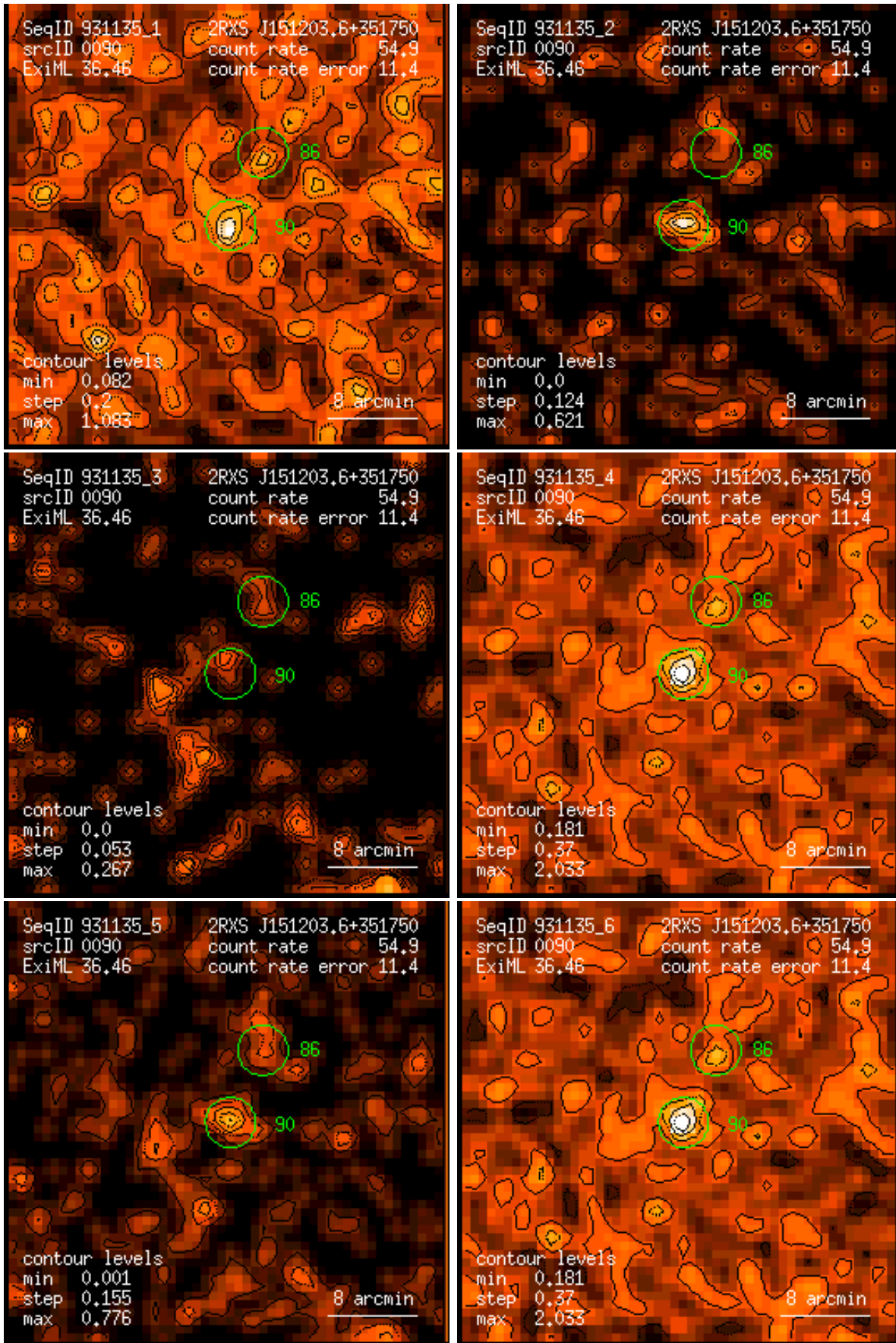
Figure 90: RASS 931135: detection 0090: band rate images, Gaussian filter: (1) PSPC channels 11 – 41, (2) 52 – 90, (3) 91 – 201, (4) 11 – 235, (5) 52 – 201, (6) 11 – 201. Broad band rates in counts/ks. Band rate contour levels in counts/ks/arcmin 2 .
