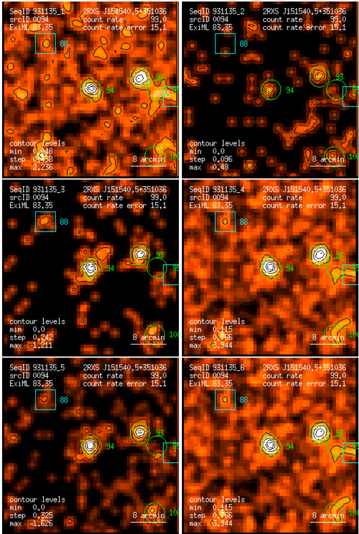
Figure 94: RASS 931135: detection 0094: band rate images, Gaussian filter: (1) PSPC channels 11 – 41, (2) 52 – 90, (3) 91 – 201, (4) 11 – 235, (5) 52 – 201, (6) 11 – 201. Broad band rates in counts/ks. Band rate contour levels in counts/ks/arcmin 2 .
