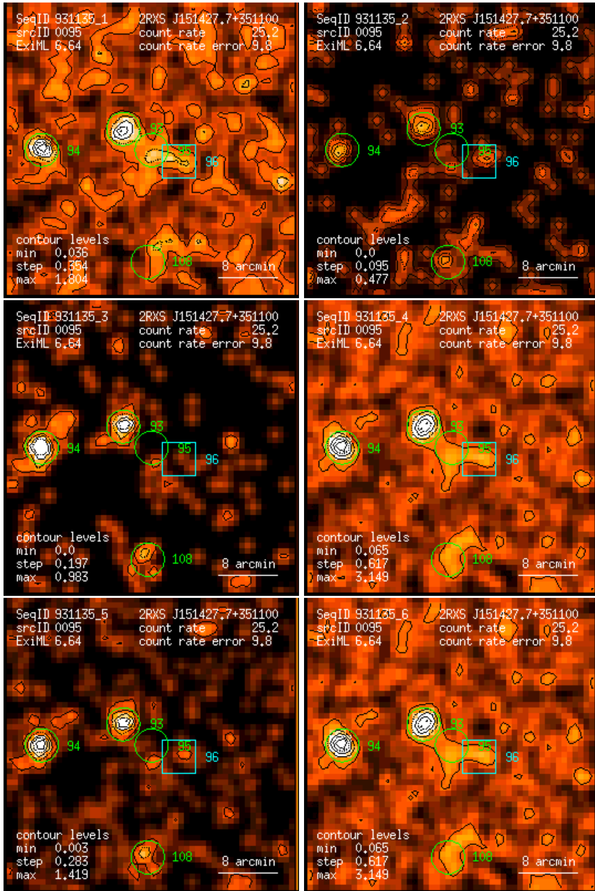
Figure 95: RASS 931135: detection 0095: band rate images, Gaussian filter: (1) PSPC channels 11 – 41, (2) 52 – 90, (3) 91 – 201, (4) 11 – 235, (5) 52 – 201, (6) 11 – 201. Broad band rates in counts/ks. Band rate contour levels in counts/ks/arcmin 2 .
