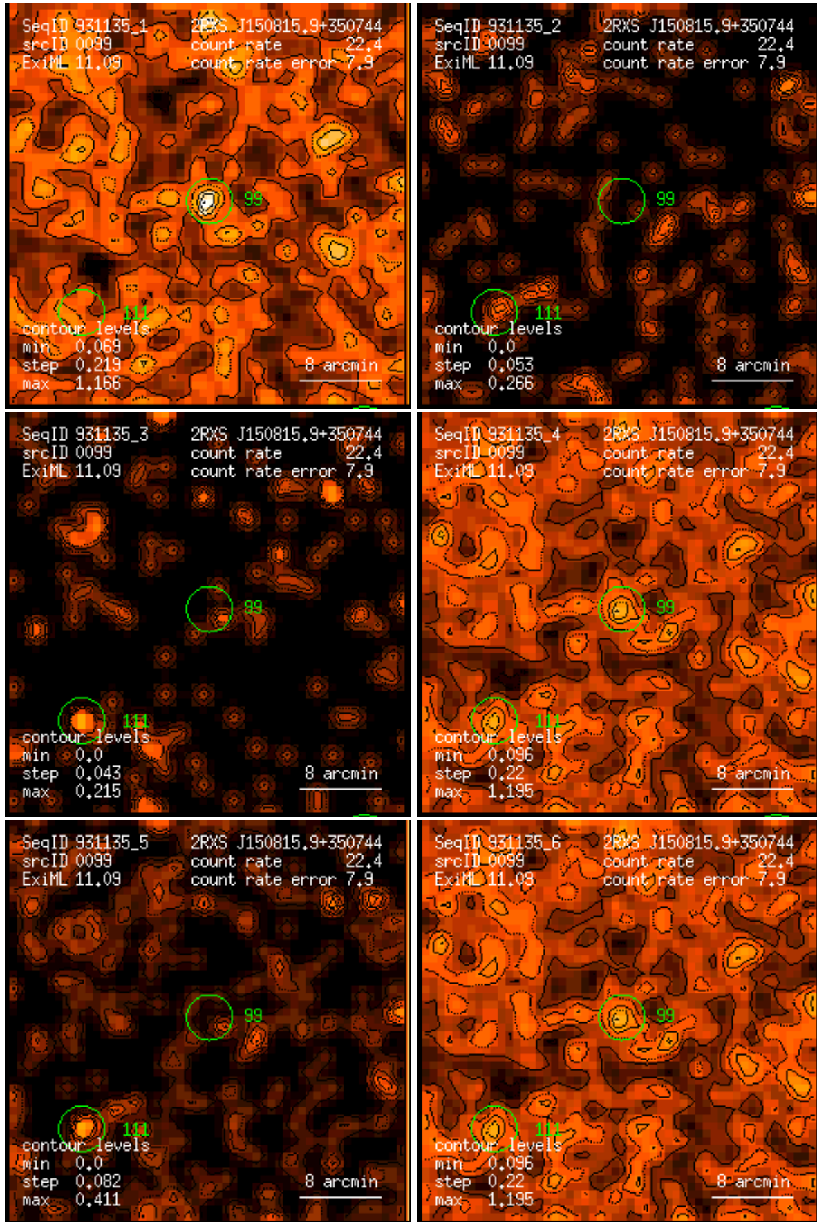
Figure 99: RASS 931135: detection 0099: band rate images, Gaussian filter: (1) PSPC channels 11 – 41, (2) 52 – 90, (3) 91 – 201, (4) 11 – 235, (5) 52 – 201, (6) 11 – 201. Broad band rates in counts/ks. Band rate contour levels in counts/ks/arcmin 2 .
